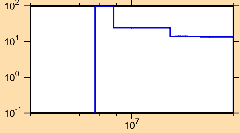
\Delta\sigma/\sigma vs. E for ^{142}\text{Pm}(n,2n)
