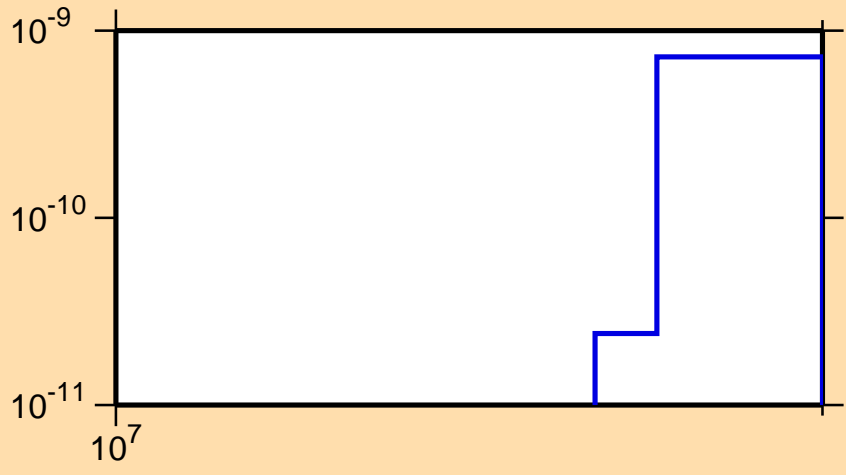
\sigma vs. E for ^{142}\text{Pm}(n,pd)
