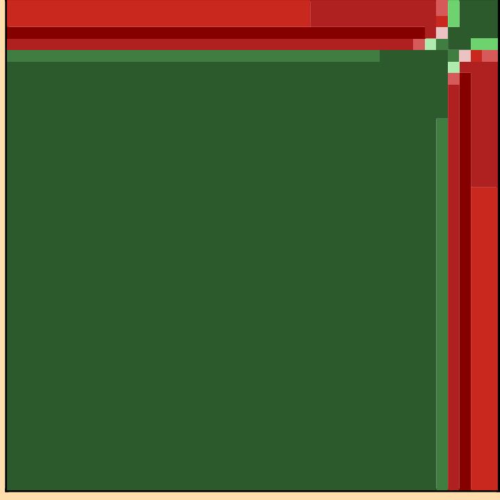
\mu vs. E for ^{142}\text{Pm}(\text{mt251})
