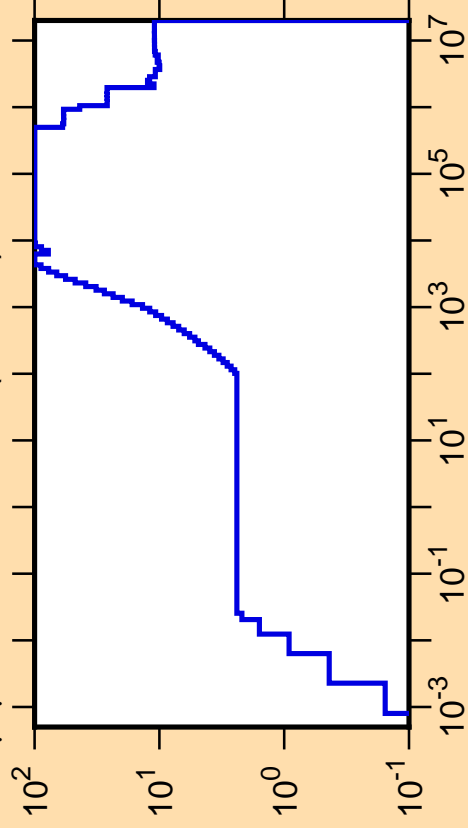
\Delta\mu/\mu vs. E for ^{143}\text{Pm}(\text{mt251})
