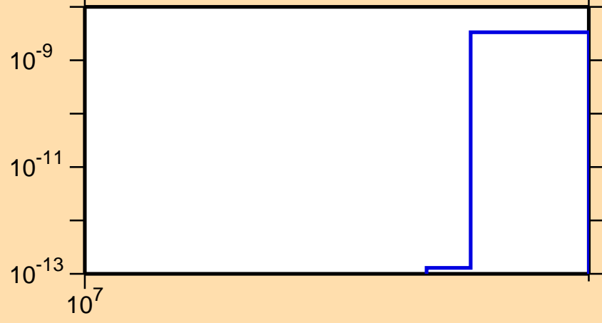
\sigma vs. E for ^{143}\text{Pm}(n,nt)
