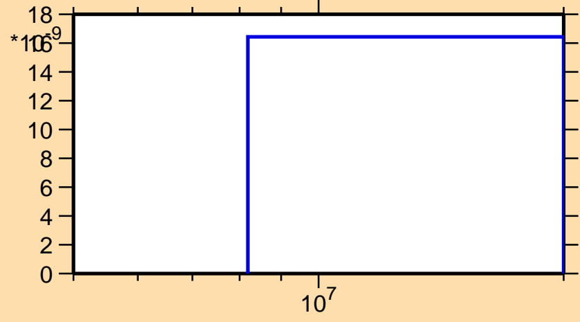
\sigma vs. E for ^{143}\text{Pm}(n,\text{nd})
