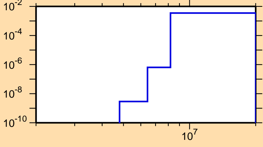
\sigma vs. E for ^{143}\text{Pm}(n,d)
