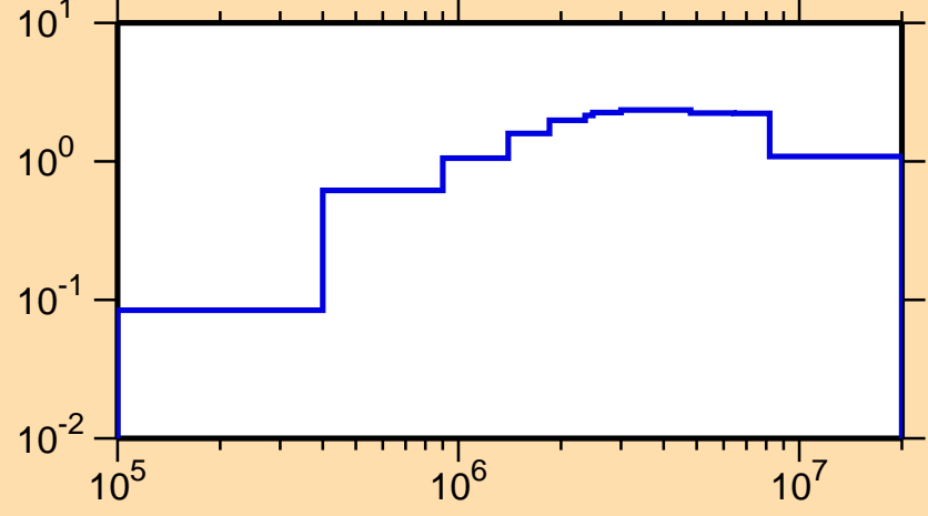
\sigma vs. E for ^{143}\text{Pm}(n,\text{inel.})
