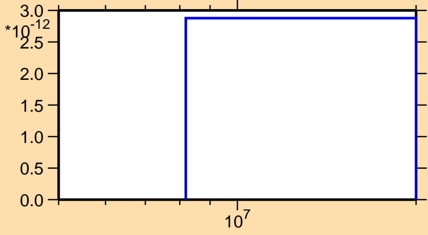
\sigma vs. E for ^{143}\text{Pm}(n,\text{pd})
