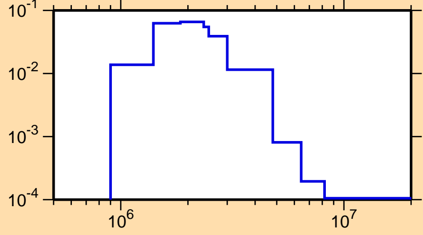
\sigma vs. E for ^{143}\text{Pm}(n,n_4)
