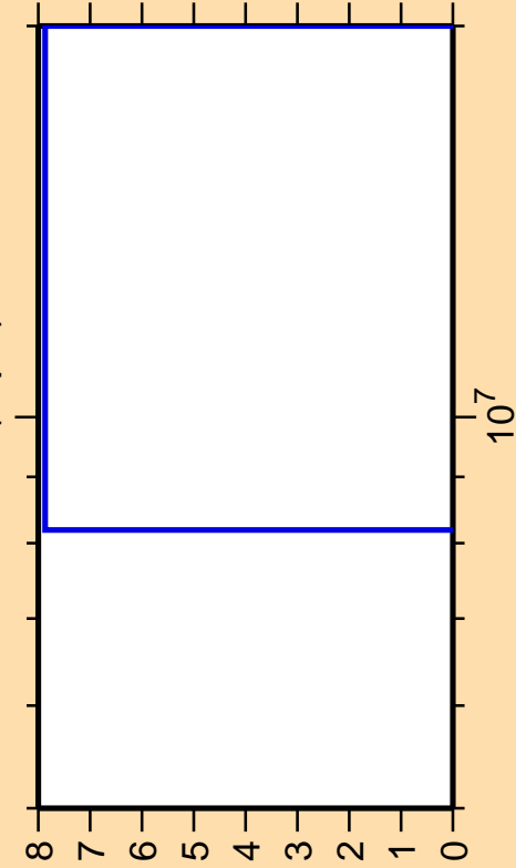
\Delta\sigma/\sigma vs. E for ^{143}\text{Pm}(n,\text{pd})
