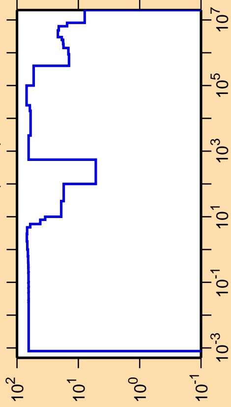
\Delta\sigma/\sigma vs. E for ^{143}\text{Pm}(n,\text{el.})
