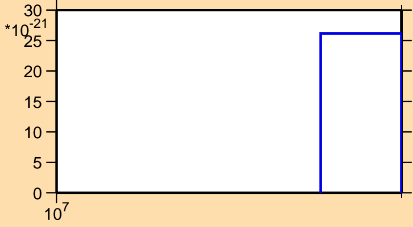
\sigma vs. E for ^{144}\text{Pm} (mt 11)
