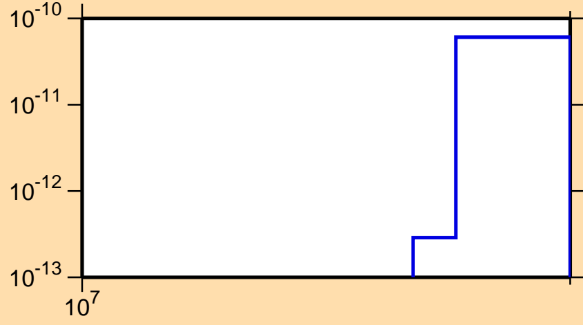
\sigma vs. E for ^{144}\text{Pm}(n,pt)
