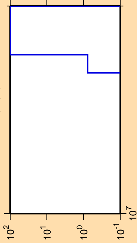
\Delta\sigma/\sigma vs. E for ^{144}\text{Pm}(n,pt)
