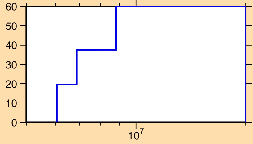
\Delta\sigma/\sigma vs. E for ^{144}\text{Pm}(n,\text{inel.})
