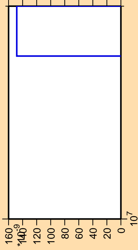
\Delta\sigma/\sigma vs. E for ^{144}\text{Pm} (mt 11)
