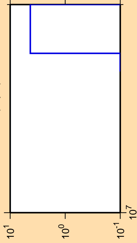
\Delta\sigma/\sigma vs. E for ^{144}\text{Pm}(n,pd)
