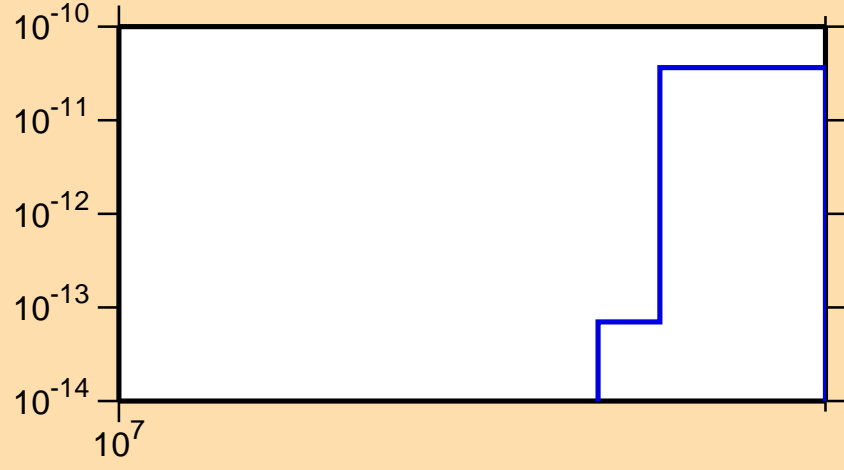
\sigma vs. E for ^{144}\text{Pm} (mt 34)
