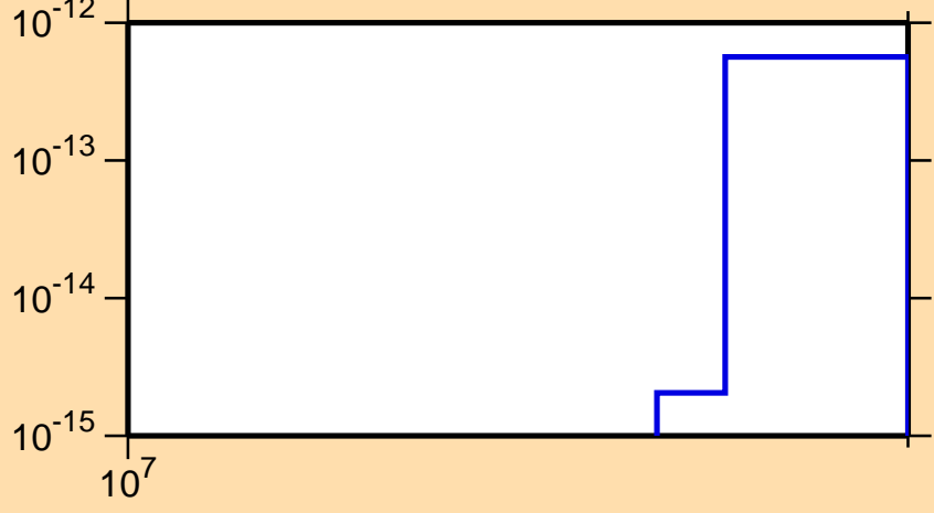
\sigma vs. E for ^{144}\text{Pm}(n,pd)
