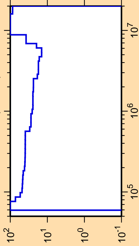
\Delta\sigma/\sigma vs. E for ^{144}\text{Pm}(n,\text{inel.})
