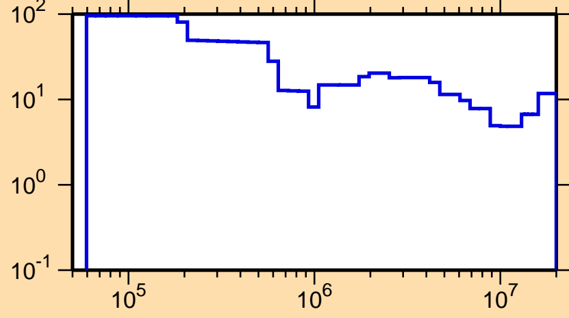
\Delta\sigma/\sigma vs. E for ^{144}\text{Pm}(n,\text{tot.})
