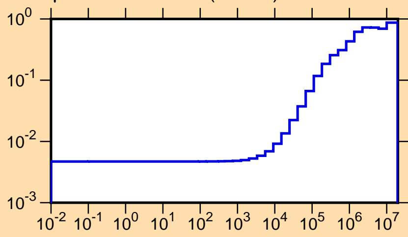
\mu vs. E for ^{144}\text{Pm}(\text{mt251})
