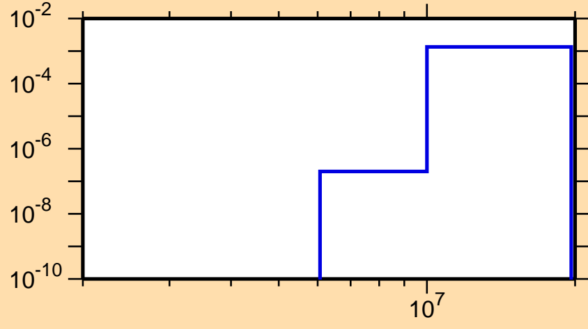
\sigma vs. E for ^{144}\text{Pm}(n,n\alpha)
