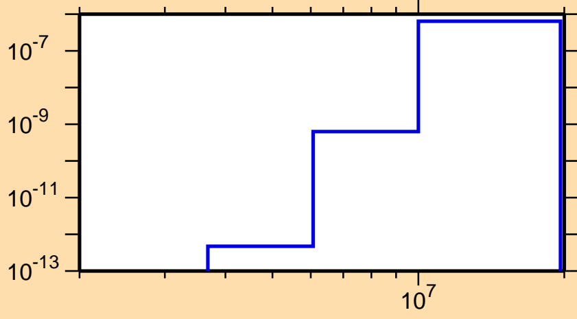
\sigma vs. E for ^{144}\text{Pm}(n,p\alpha)
