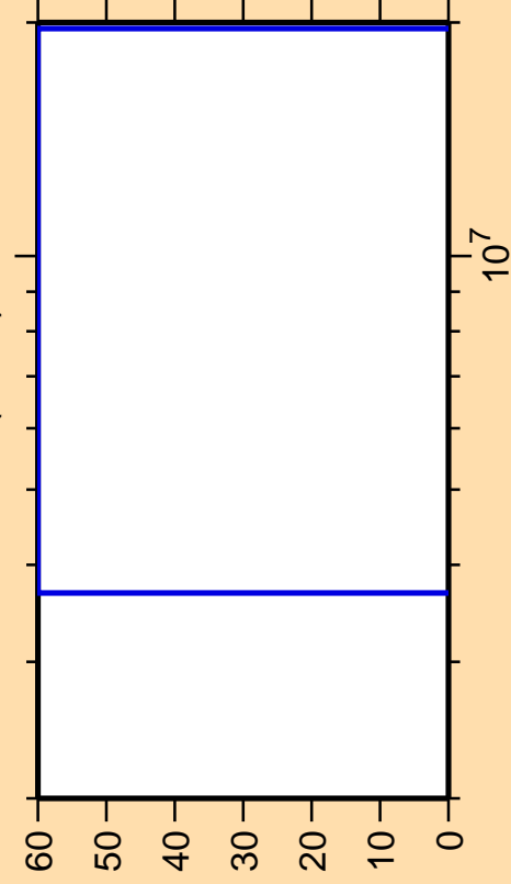
\Delta\sigma/\sigma vs. E for ^{144}\text{Pm}(n,n\alpha)
