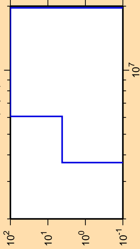
\Delta\sigma/\sigma vs. E for ^{144}\text{Pm}(n,p\alpha)
