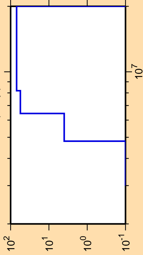
\Delta\sigma/\sigma vs. E for ^{144}\text{Pm}(n,np)
