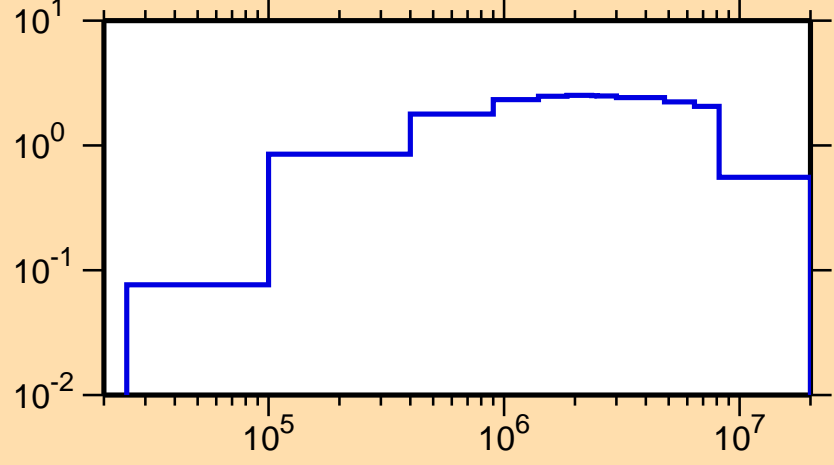
\sigma vs. E for ^{144}\text{Pm}(n,\text{inel.})
