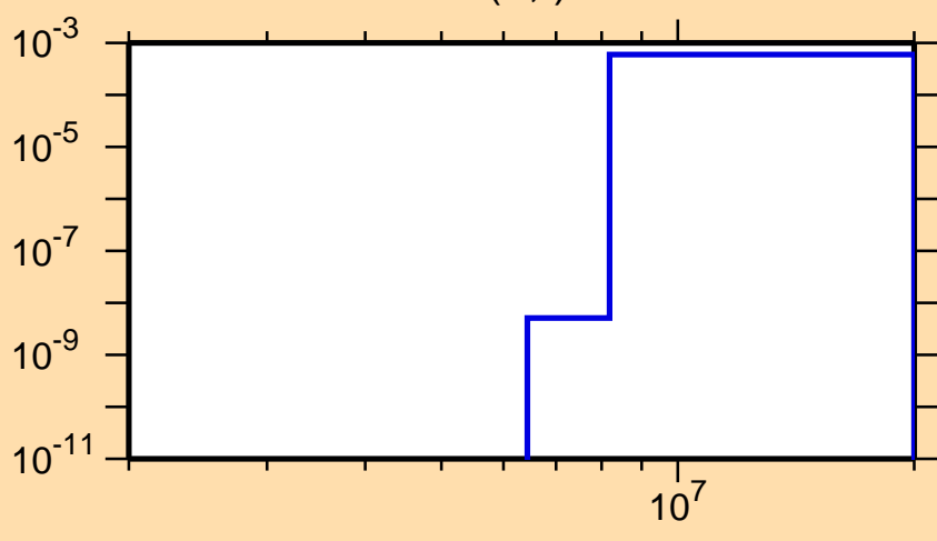
\sigma vs. E for ^{144}\text{Pm}(n,t)
