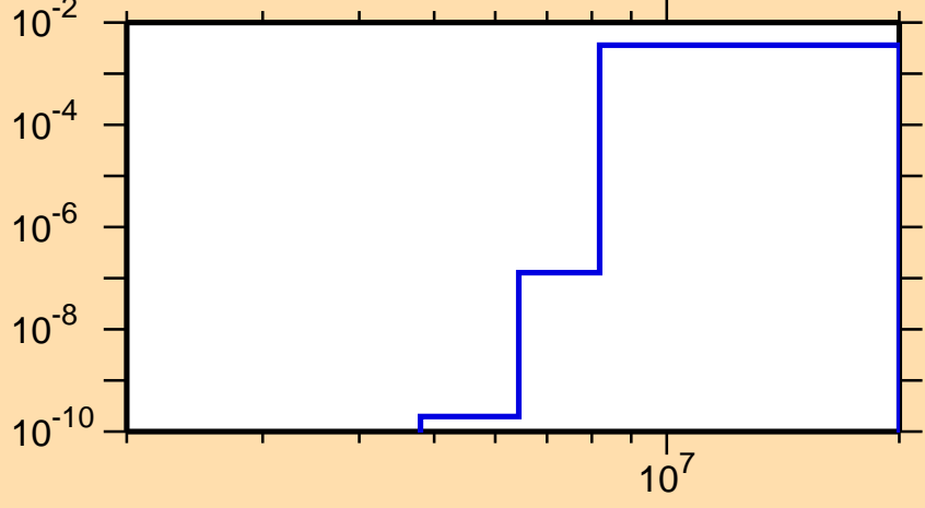
\sigma vs. E for ^{144}\text{Pm}(n,d)
