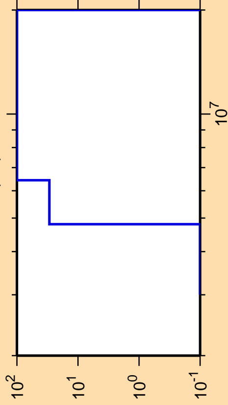
\Delta\sigma/\sigma vs. E for ^{144}\text{Pm}(n,t)
