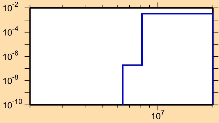
\sigma vs. E for ^{144}\text{Pm}(n,np)
