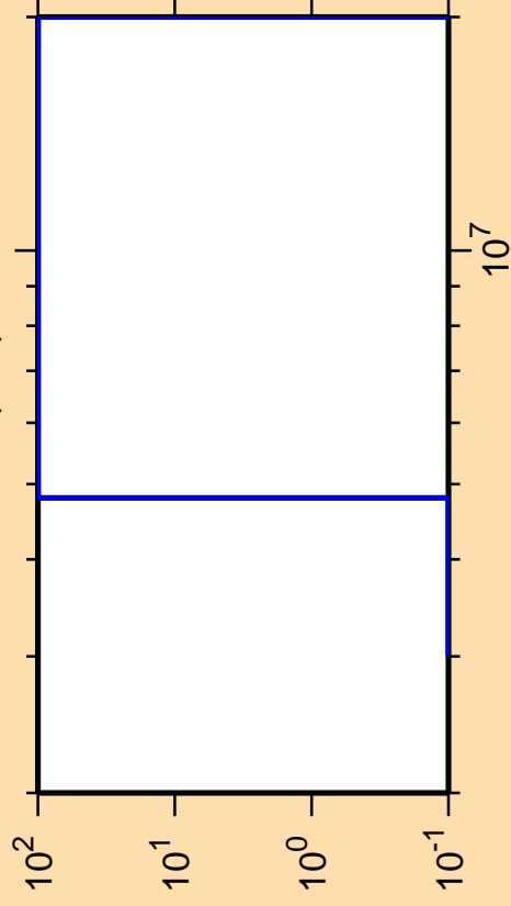
\Delta\sigma/\sigma vs. E for ^{144}\text{Pm}(n,d)
