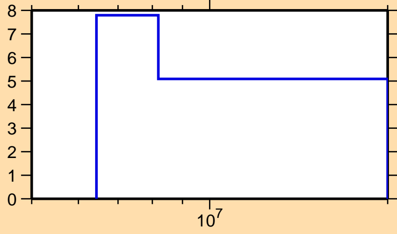
\Delta\sigma/\sigma vs. E for ^{144}\text{Pm}(n,\text{tot.})
