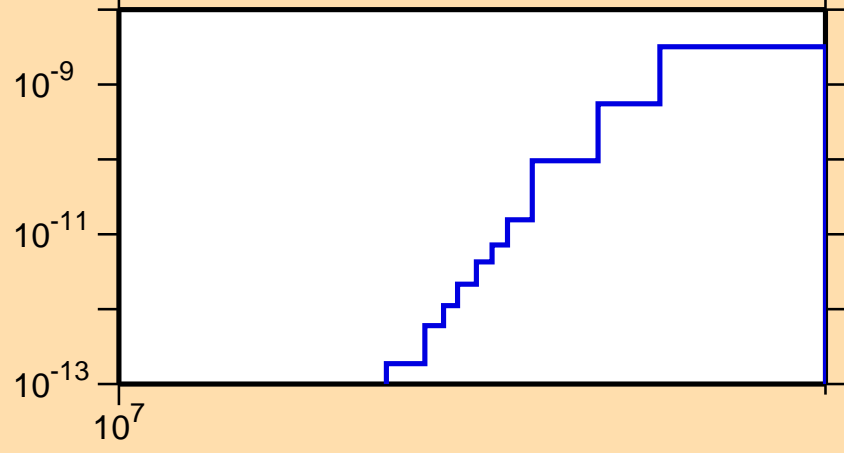
\sigma vs. E for ^{145}\text{Pm} (mt 45)
