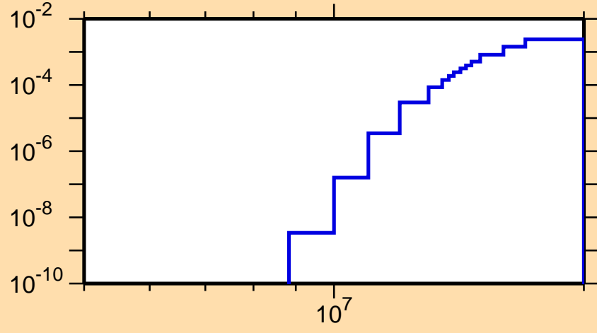
\sigma vs. E for ^{145}\text{Pm}(n,t)
