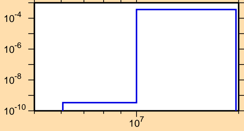
\sigma vs. E for ^{145}\text{Pm}(n,t)
