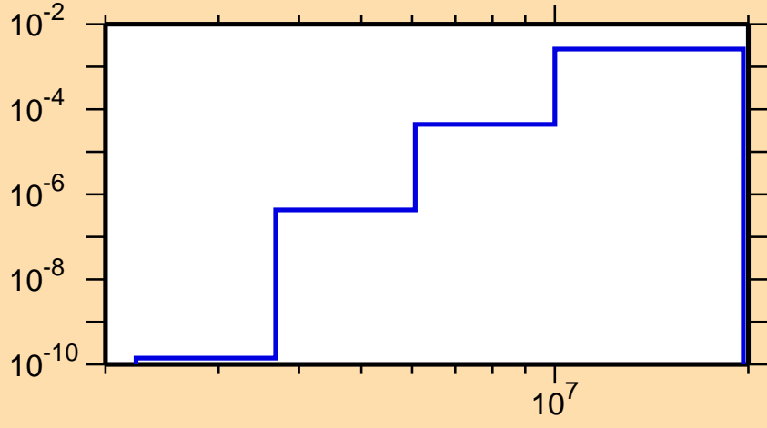
\sigma vs. E for ^{145}\text{Pm}(n,\alpha)
