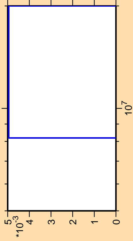
\Delta\sigma/\sigma vs. E for ^{145}\text{Pm} (mt 34)
