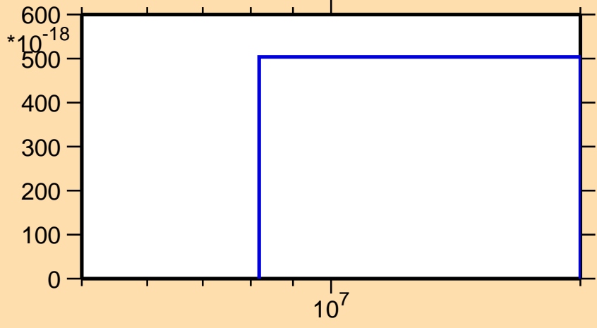
\sigma vs. E for ^{145}\text{Pm}(n,pd)
