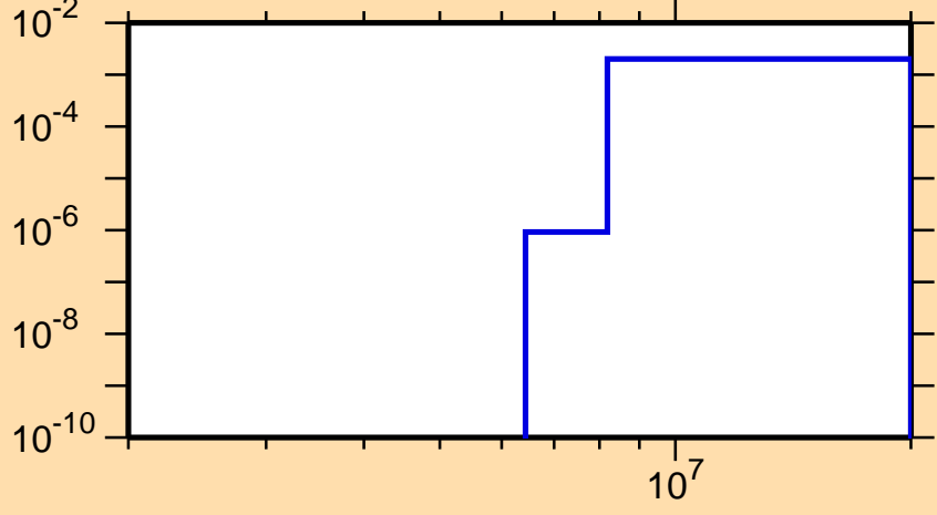
\sigma vs. E for ^{145}\text{Pm}(n,np)
