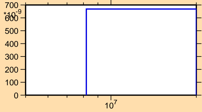
\sigma vs. E for ^{145}\text{Pm}(n,nd)
