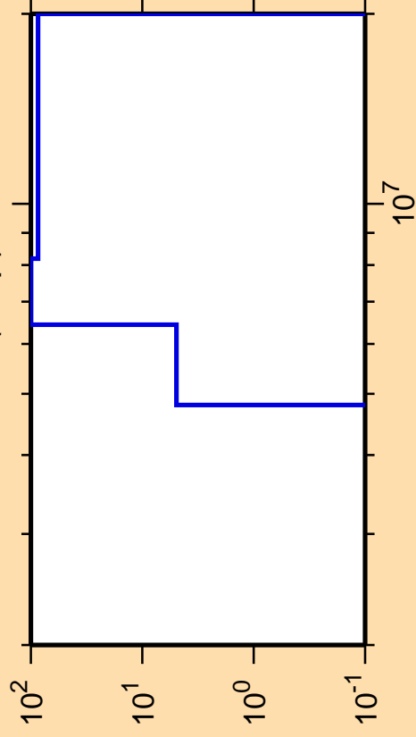
\Delta\sigma/\sigma vs. E for ^{145}\text{Pm}(n,np)
