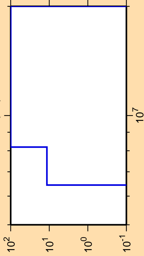
\Delta\sigma/\sigma vs. E for ^{145}\text{Pm}(n,t)
