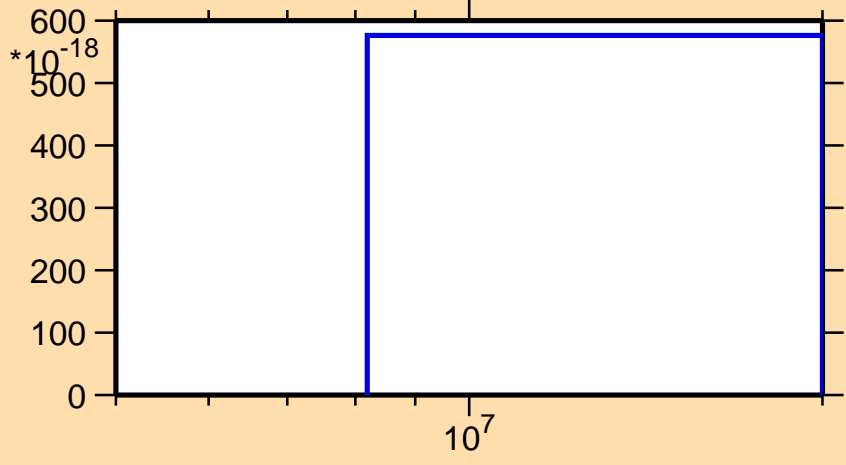
\sigma vs. E for ^{145}\text{Pm} (mt 11)
