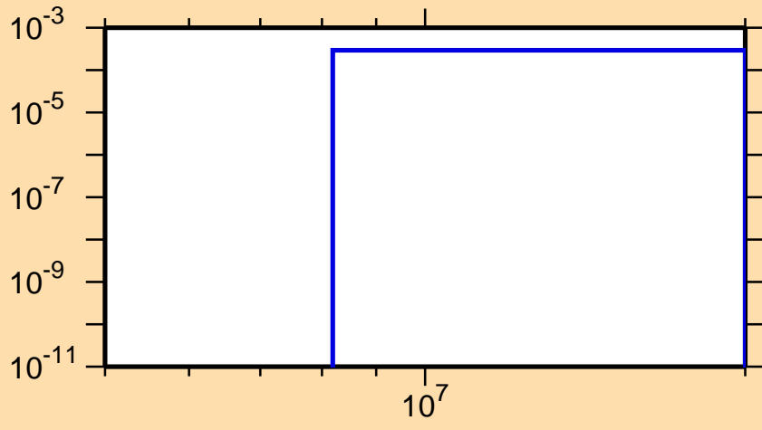
\sigma vs. E for ^{145}\text{Pm}(n,t)
