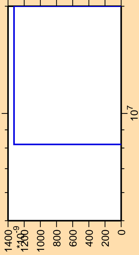
\Delta\sigma/\sigma vs. E for ^{145}\text{Pm} (mt 42)
