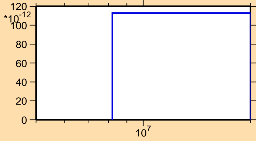
\sigma vs. E for ^{145}\text{Pm}(\text{mt117})
