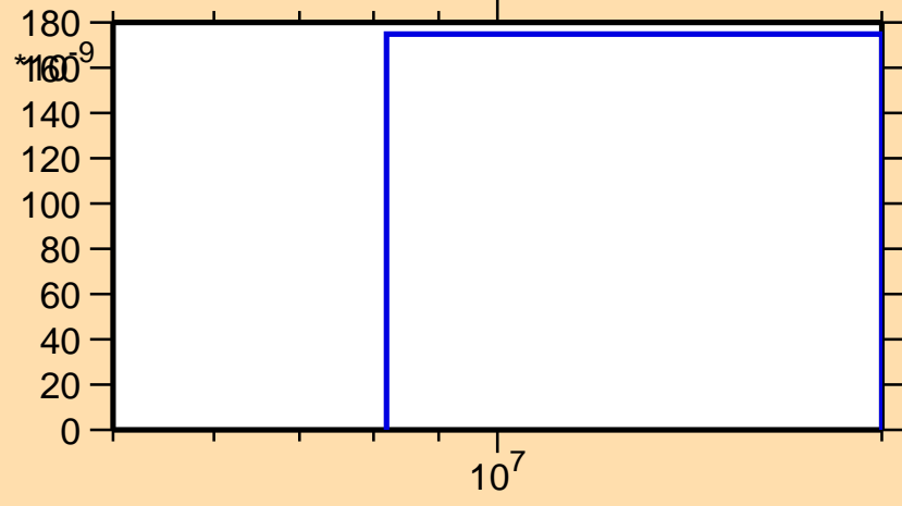
\sigma vs. E for ^{145}\text{Pm}(n,nt)
