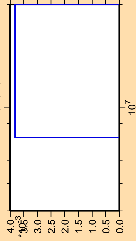
\Delta\sigma/\sigma vs. E for ^{145}\text{Pm}(n,pd)
