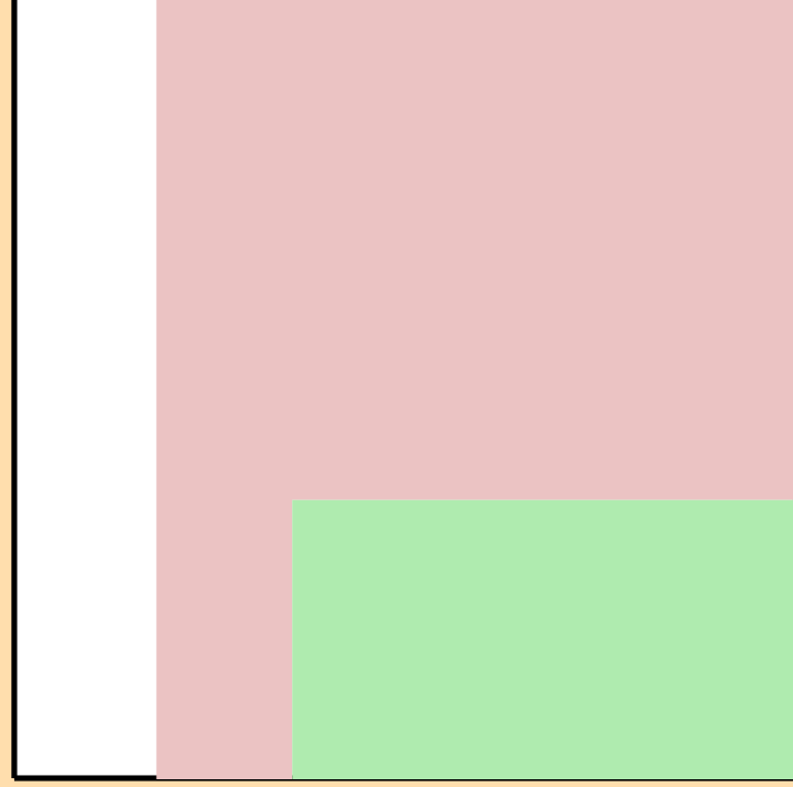
\Delta\sigma/\sigma vs. E for ^{145}\text{Pm}(n,2n)
