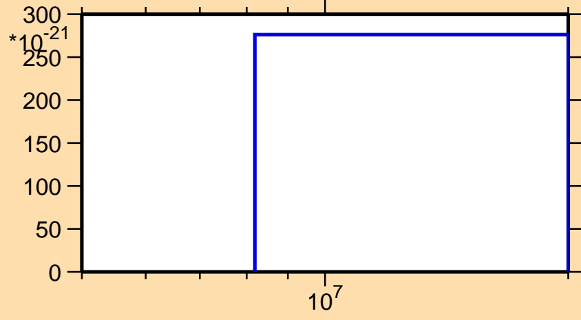
\sigma vs. E for ^{145}\text{Pm} (mt 42)
