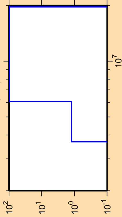
\Delta\sigma/\sigma vs. E for ^{146}\text{Pm}(n,d)
