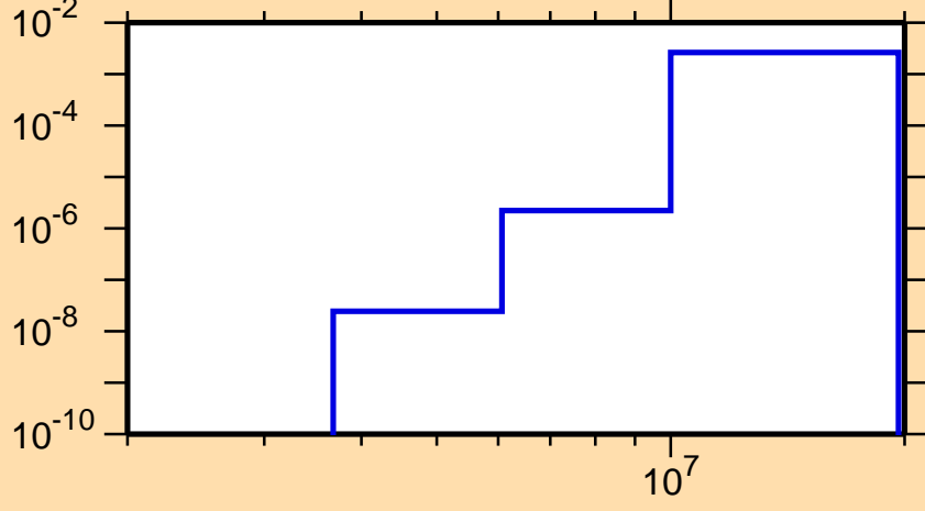
\sigma vs. E for ^{146}\text{Pm}(n,n\alpha)
