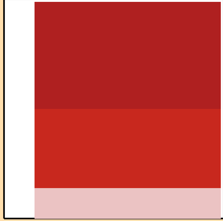
\Delta\sigma/\sigma vs. E for ^{146}\text{Pm}(n,2n)
