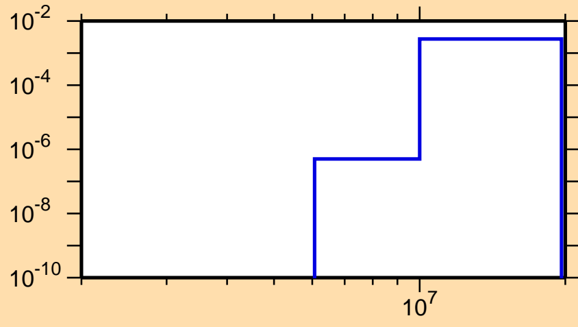
\sigma vs. E for ^{146}\text{Pm}(n,d)
