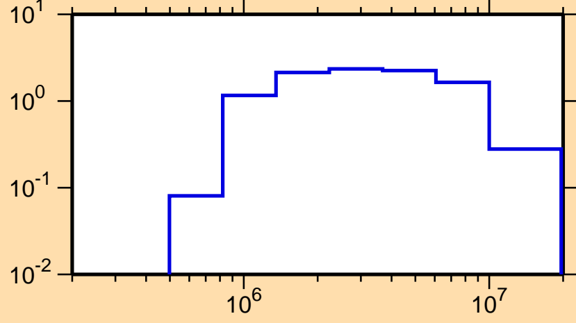
\sigma vs. E for ^{146}\text{Pm}(n,n\text{cont.})
