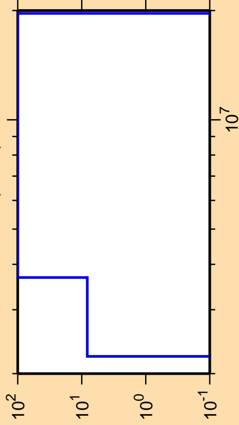
\Delta\sigma/\sigma vs. E for ^{146}\text{Pm}(n,n\alpha)
