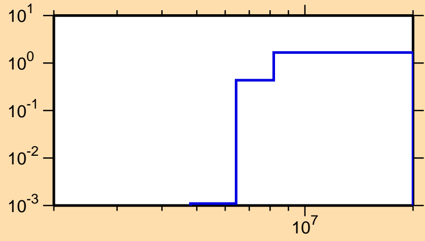
\sigma vs. E for ^{146}\text{Pm}(n,2n)
