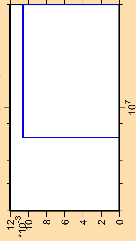
\Delta\sigma/\sigma vs. E for ^{146}\text{Pm} (mt 11)
