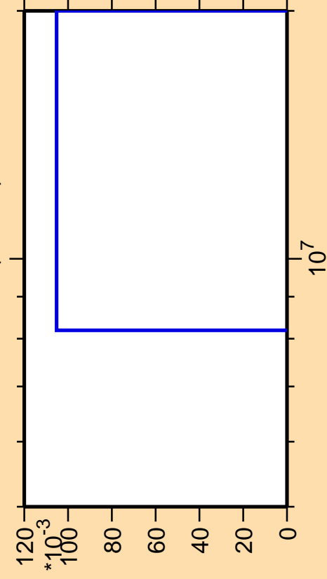
\Delta\sigma/\sigma vs. E for ^{146}\text{Pm} (mt 34)
