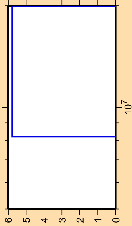
\Delta\sigma/\sigma vs. E for ^{146}\text{Pm} (mt 45)
