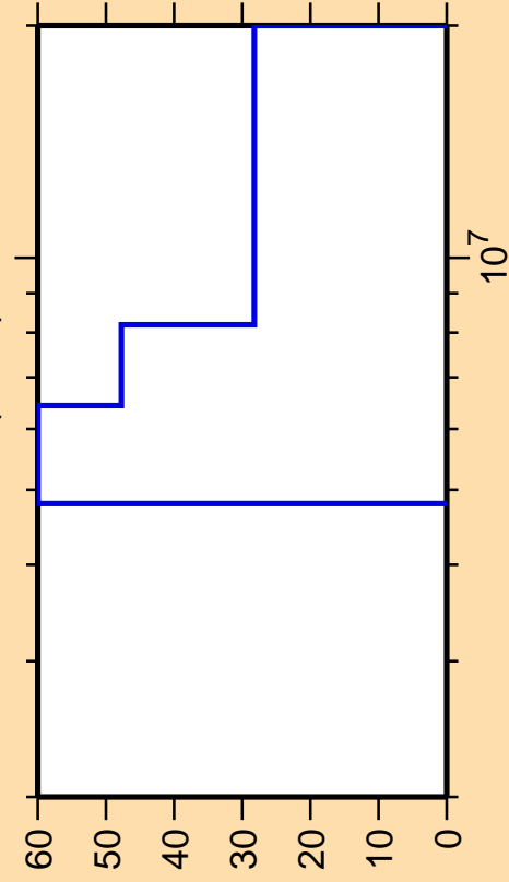
\Delta\sigma/\sigma vs. E for ^{146}\text{Pm}(n,2n)
