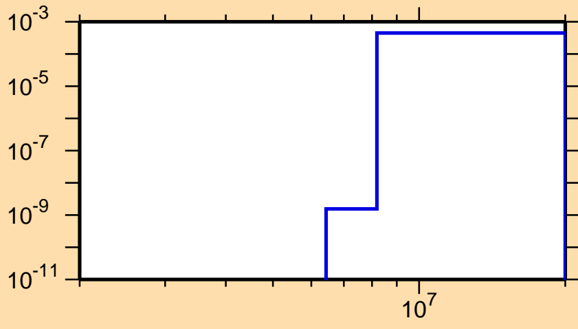
\sigma vs. E for ^{146}\text{Pm}(n,t)
