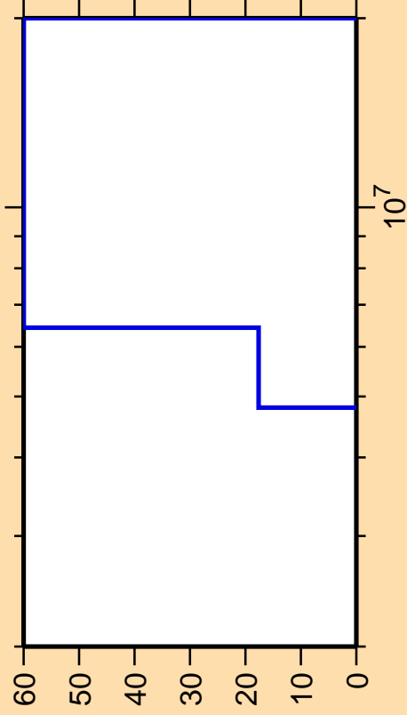
\Delta\sigma/\sigma vs. E for ^{146}\text{Pm}(n,n\text{cont.})
