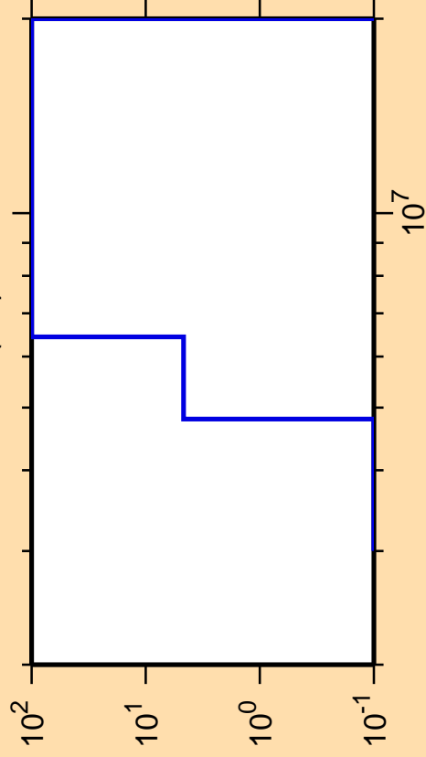
\Delta\sigma/\sigma vs. E for ^{146}\text{Pm}(n,t)
