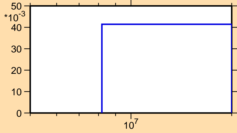
\sigma vs. E for ^{146}\text{Pm}(n,3n)
