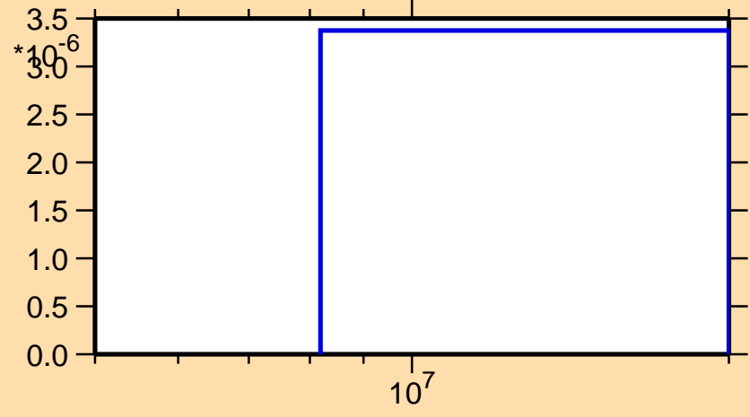
\sigma vs. E for ^{146}\text{Pm}(n,\text{nd})
