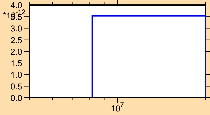
\sigma vs. E for ^{146}\text{Pm}(\text{mt117})
