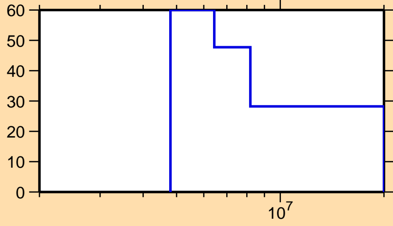
\Delta\sigma/\sigma vs. E for ^{146}\text{Pm}(n,2n)
