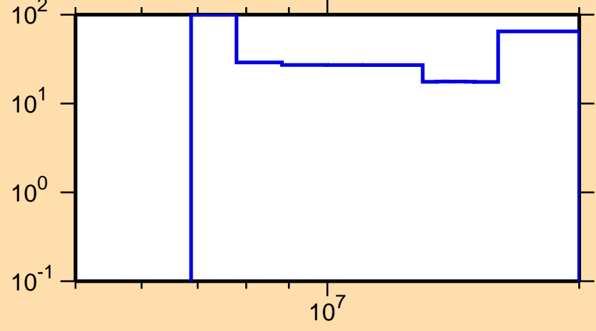
\Delta\sigma/\sigma vs. E for ^{147}\text{Pm}(n,2n)
