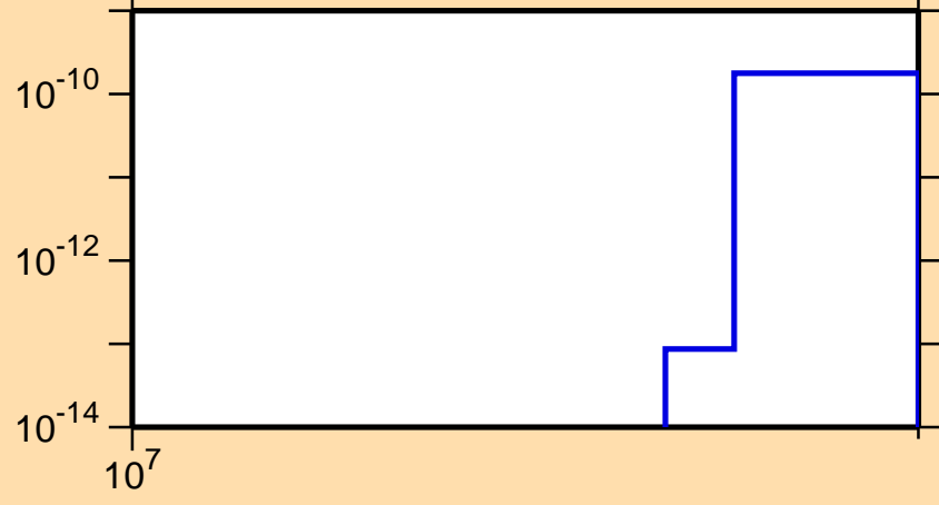
\sigma vs. E for ^{147}\text{Pm}(n,3n\alpha)
