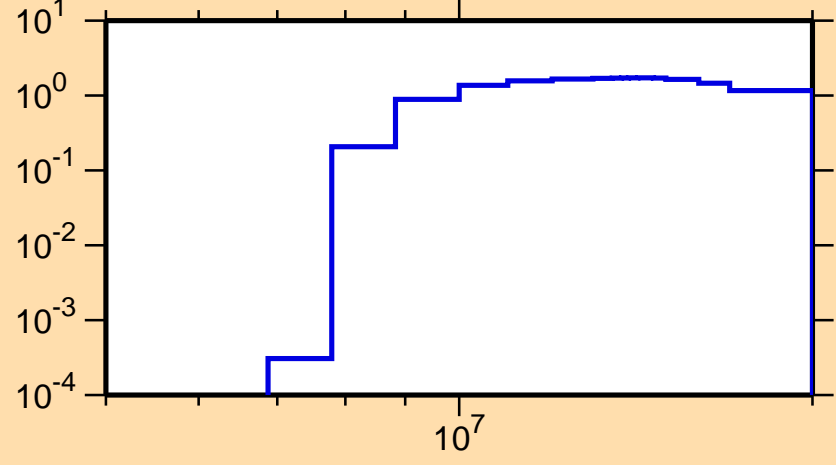
\sigma vs. E for ^{147}\text{Pm}(n,2n)
