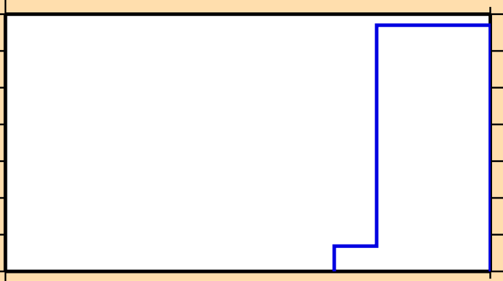
\sigma vs. E for ^{147}\text{Pm} (mt 45)
