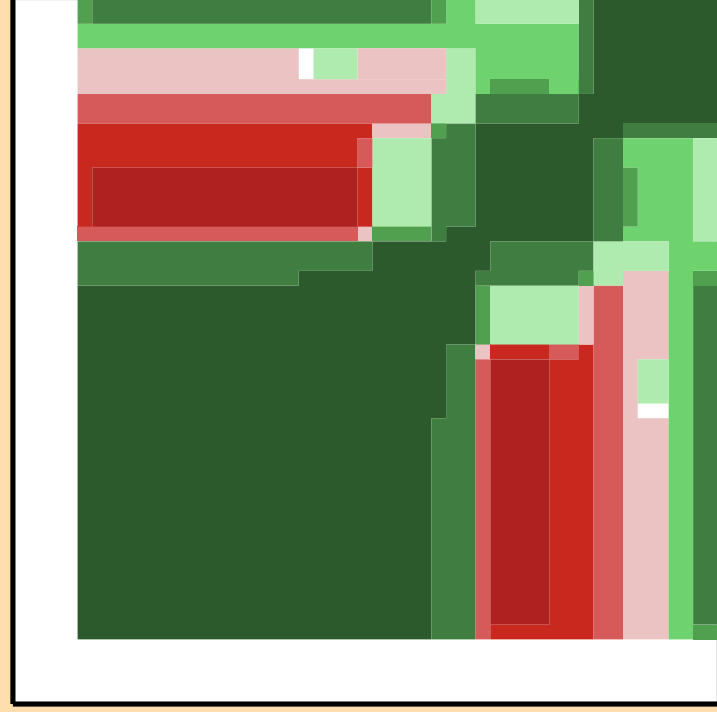
\sigma vs. E for ^{147}\text{Pm}(n,\text{inel.})
