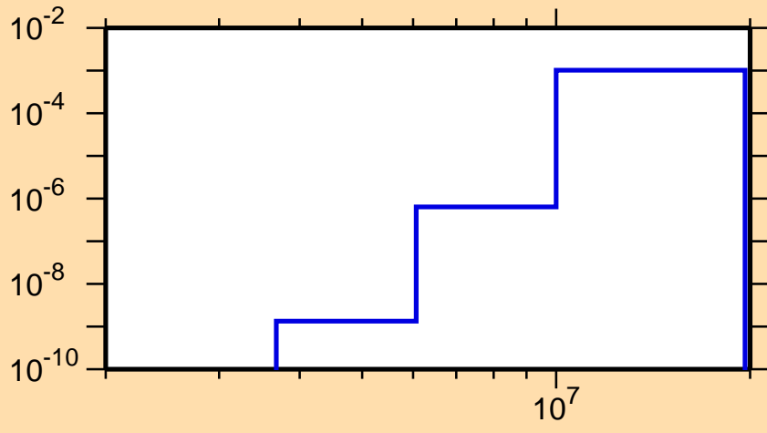
\sigma vs. E for ^{147}\text{Pm}(n,n\alpha)
