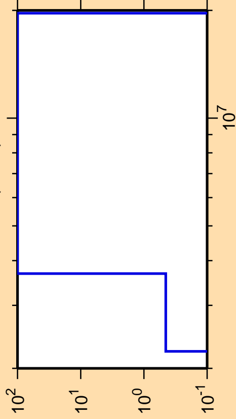
\Delta\sigma/\sigma vs. E for ^{147}\text{Pm}(n,n\alpha)
