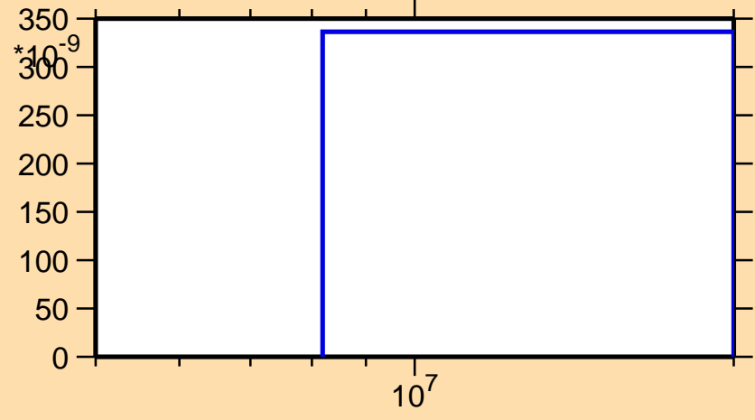
\sigma vs. E for ^{147}\text{Pm}(n,\text{nd})
