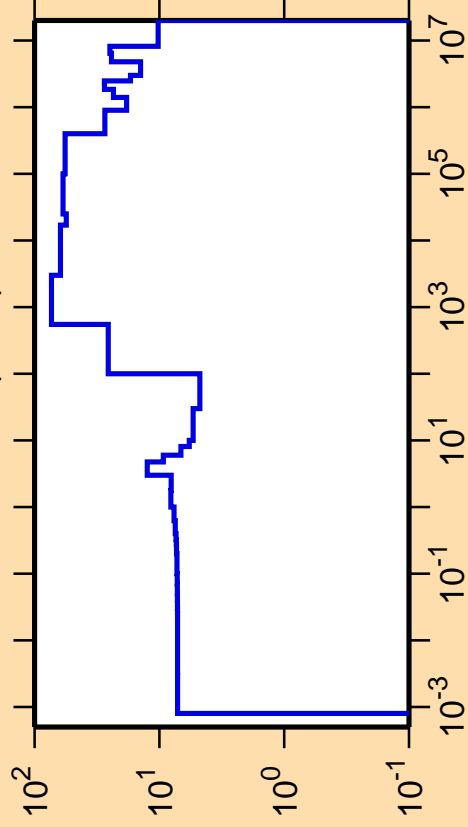
\Delta\sigma/\sigma vs. E for ^{147}\text{Pm}(n,\text{el.})
