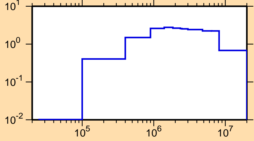
\sigma vs. E for ^{147}\text{Pm}(n,\text{inel.})
