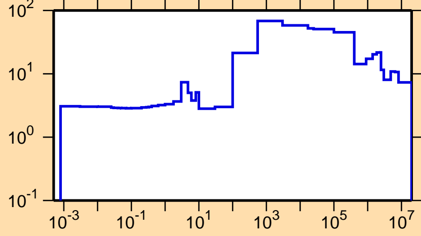
\Delta\sigma/\sigma vs. E for ^{147}\text{Pm}(n,\text{tot.})
