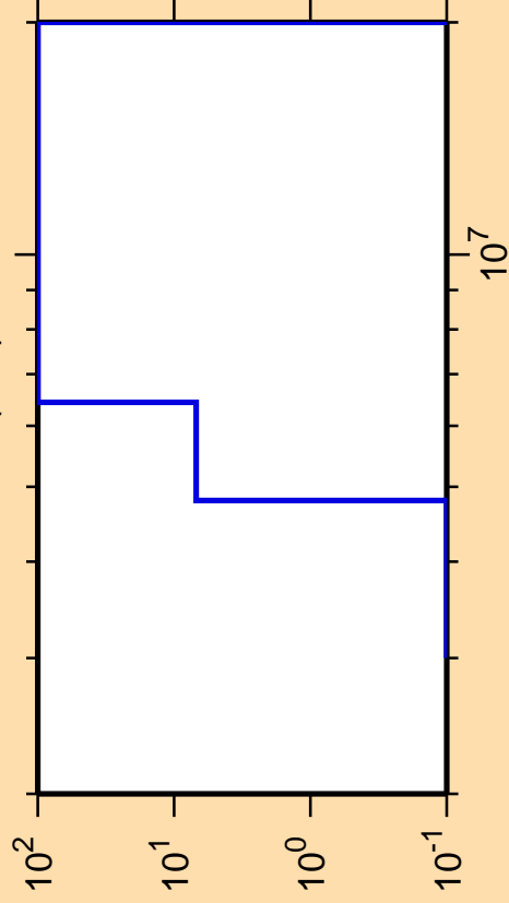
\Delta\sigma/\sigma vs. E for ^{147}\text{Pm}(n,d)
