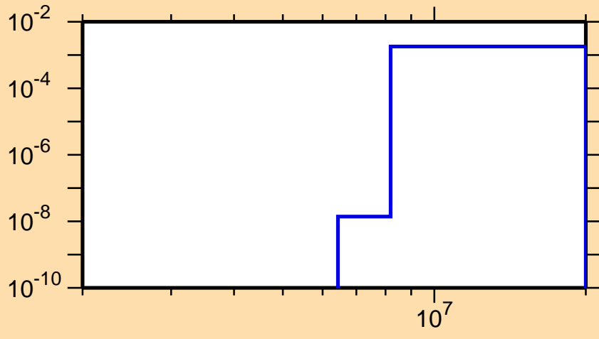
\sigma vs. E for ^{147}\text{Pm}(n,d)
