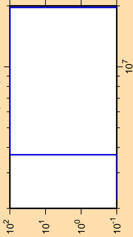
\Delta\sigma/\sigma vs. E for ^{148}\text{Pm}(n,n\alpha)
