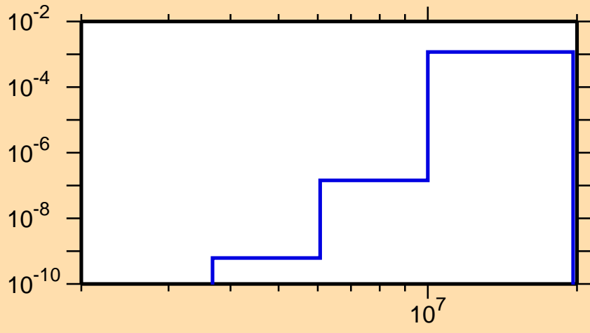
\sigma vs. E for ^{148}\text{Pm}(n,n\alpha)
