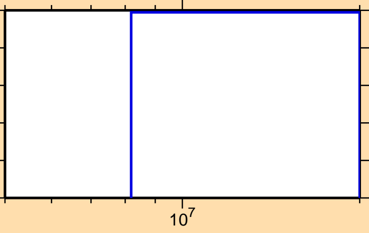
\sigma vs. E for ^{148}\text{Pm}(n,nt)
