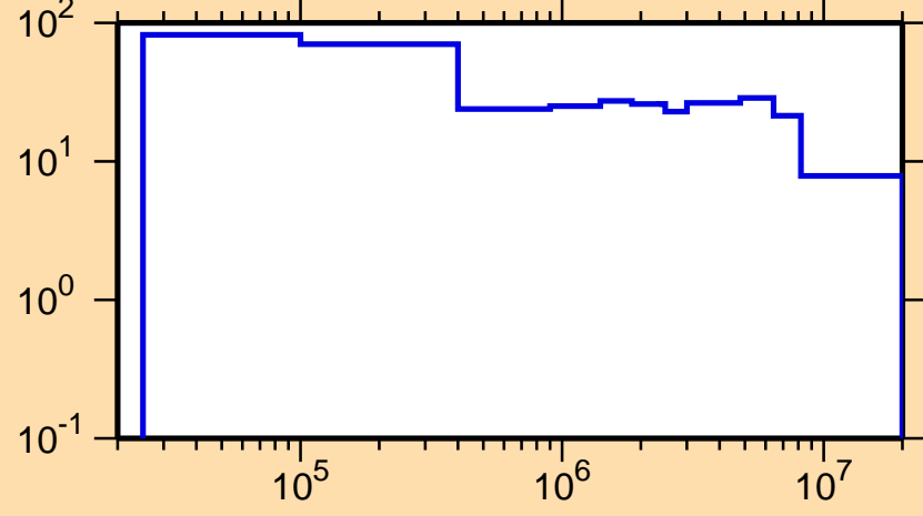
\Delta\sigma/\sigma vs. E for ^{148}\text{Pm}(n,\text{tot.})
