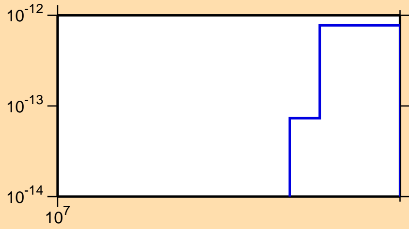
\sigma vs. E for ^{148}\text{Pm} (mt 45)
