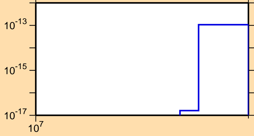
\sigma vs. E for ^{148}\text{Pm} (mt 34)
