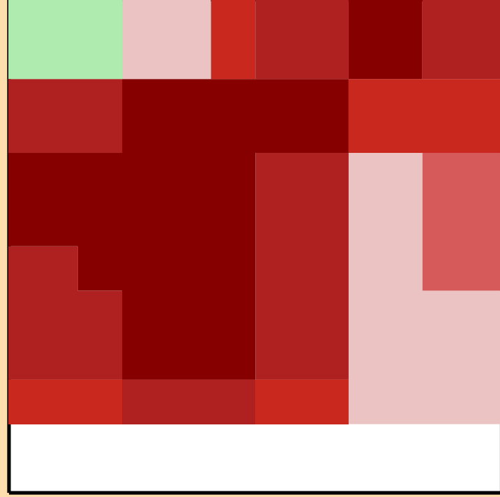
\Delta\sigma/\sigma vs. E for ^{148}\text{Pm}(n,\text{el.})
