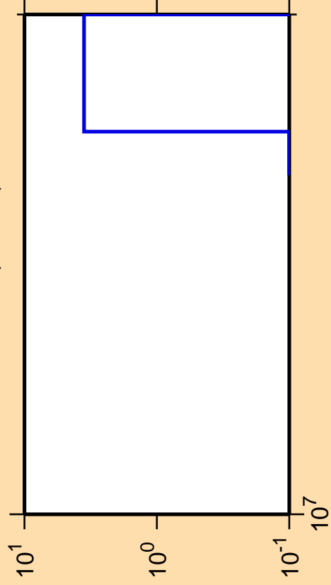
\Delta\sigma/\sigma vs. E for ^{149}\text{Pm} (mt 11)
