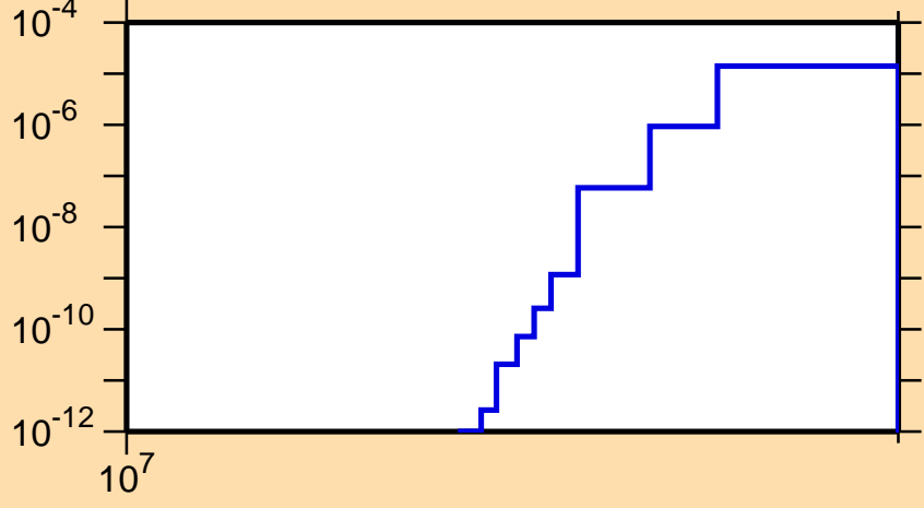
\sigma vs. E for ^{149}\text{Pm}(n,\text{nd})
