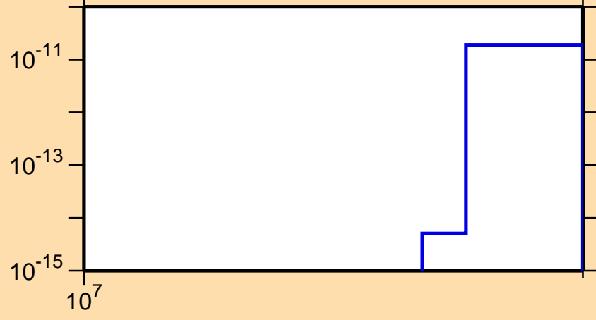
\sigma vs. E for ^{149}\text{Pm}(n,3n\alpha)
