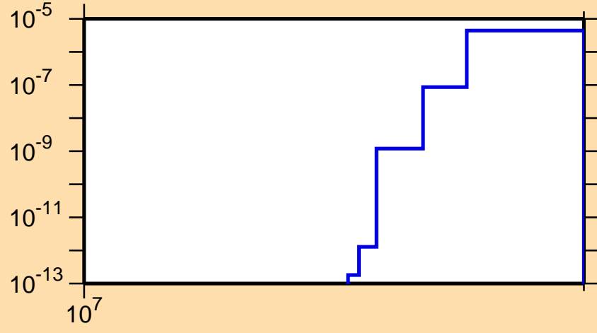
\sigma vs. E for ^{149}\text{Pm}(n,2np)
