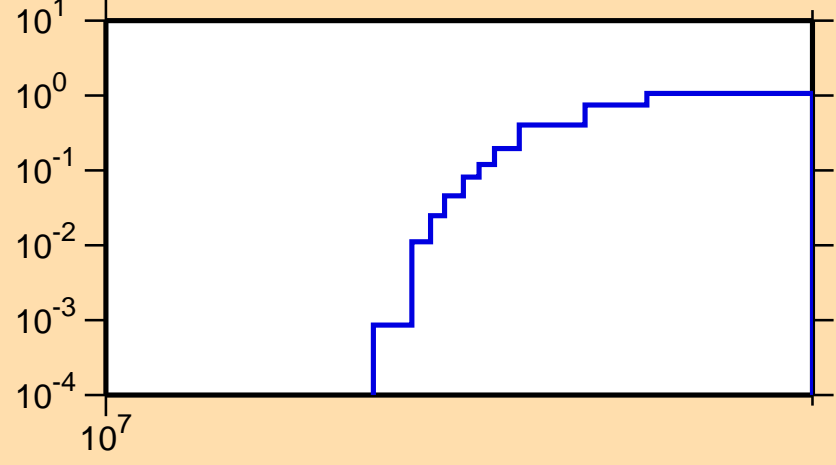
\sigma vs. E for ^{149}\text{Pm}(n,3n)
