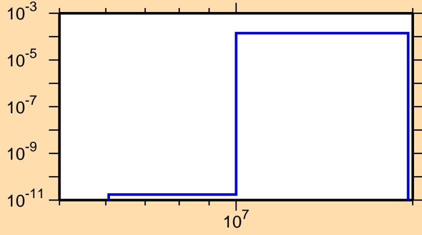
\sigma vs. E for ^{149}\text{Pm}(n,t)
