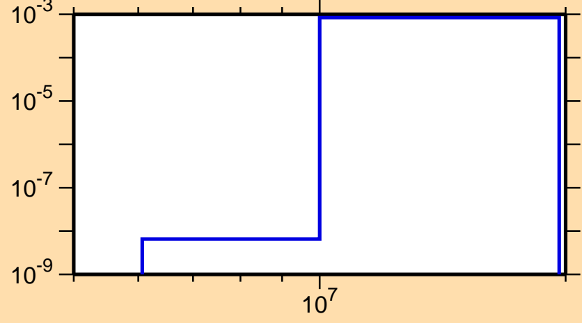
\sigma vs. E for ^{149}\text{Pm}(n,np)
