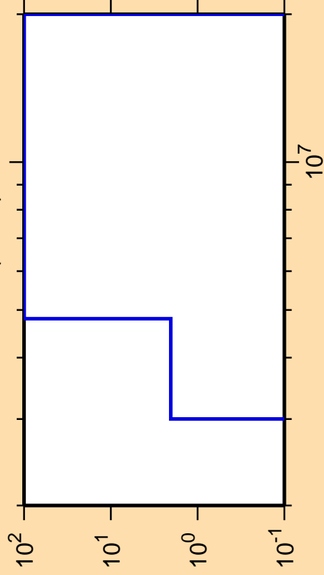
\Delta\sigma/\sigma vs. E for ^{149}\text{Pm}(n,n\alpha)
