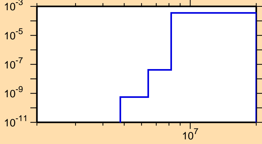
\sigma vs. E for ^{149}\text{Pm}(n,n\alpha)
