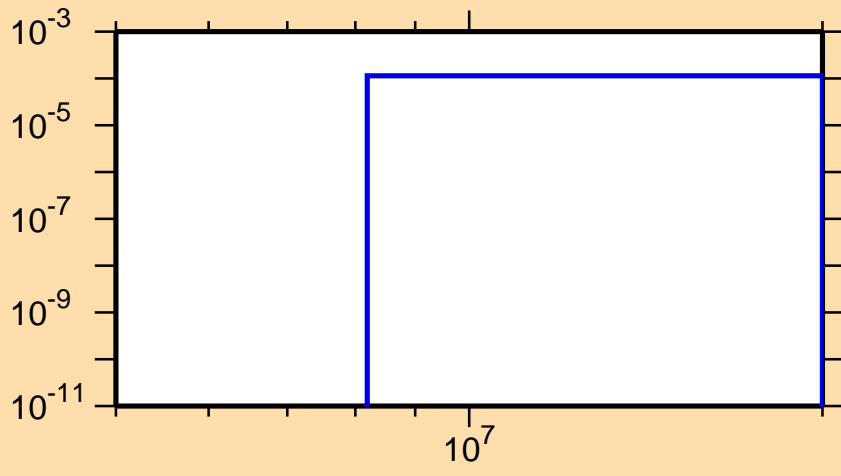
\sigma vs. E for ^{149}\text{Pm}(n,t)
