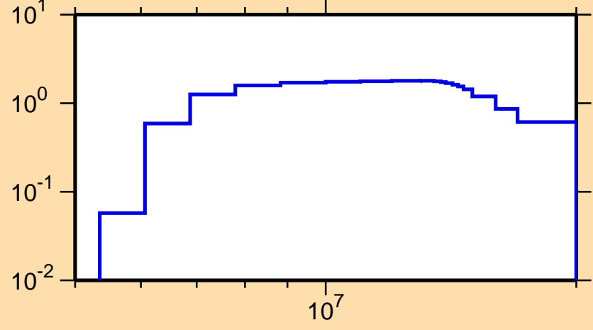
\sigma vs. E for ^{150}\text{Pm}(n,2n)
