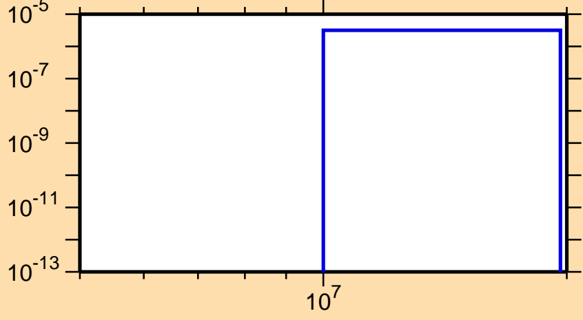
\sigma vs. E for ^{150}\text{Pm}(n,\text{nd})
