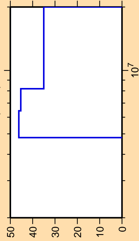
\Delta\sigma/\sigma vs. E for ^{150}\text{Pm}(n,2n)
