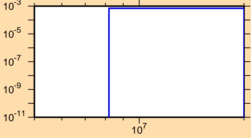
\sigma vs. E for ^{150}\text{Pm}(n,np)
