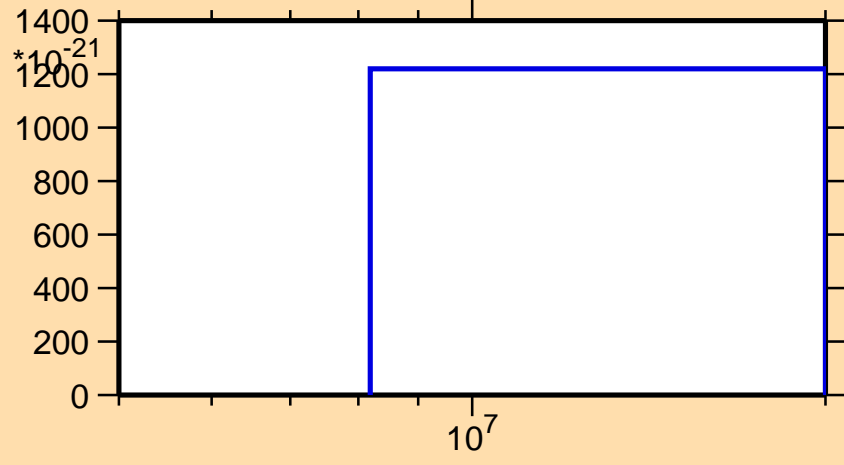
\sigma vs. E for ^{150}\text{Pm} (mt 42)
