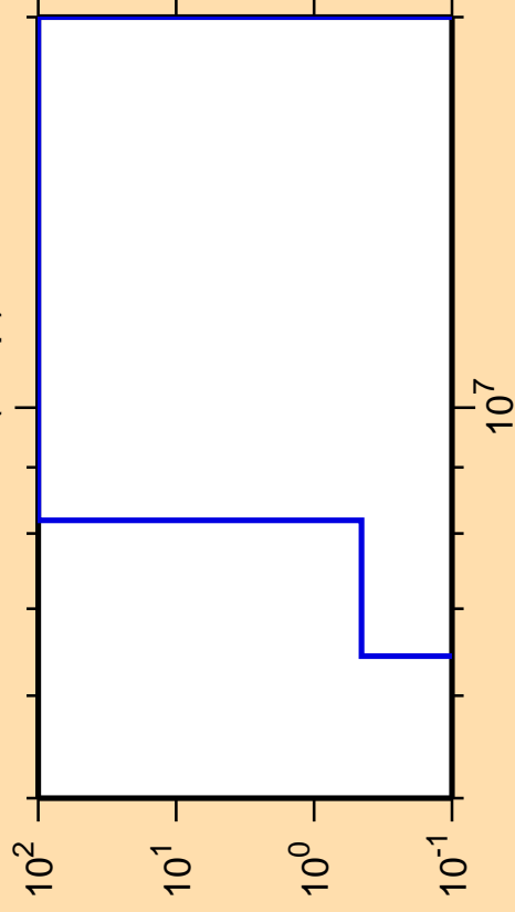
\Delta\sigma/\sigma vs. E for ^{150}\text{Pm}(n,np)
