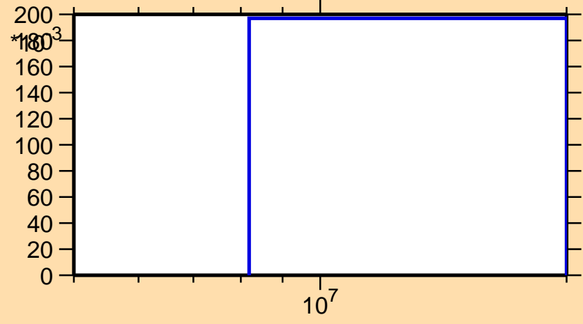
\sigma vs. E for ^{150}\text{Pm}(n,3n)
