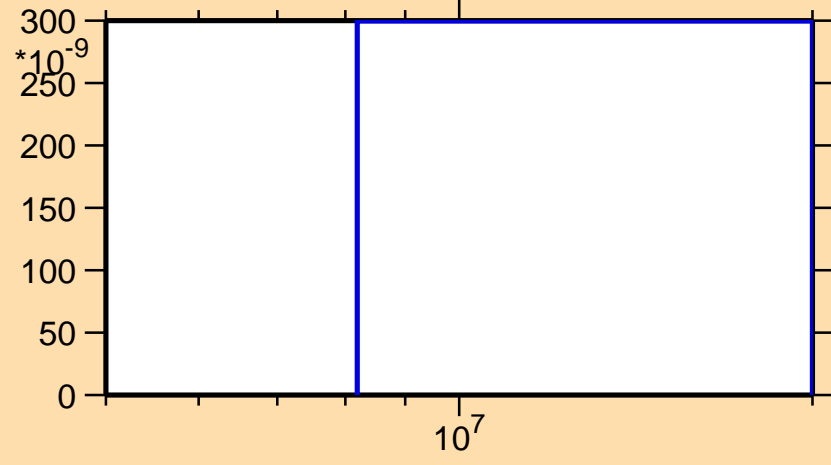
\sigma vs. E for ^{150}\text{Pm}(n,2n\alpha)
