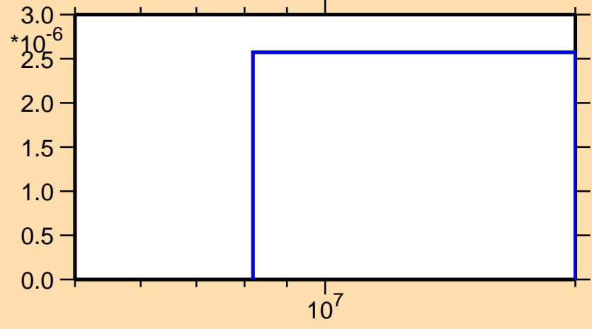
\sigma vs. E for ^{150}\text{Pm}(n,nd)
