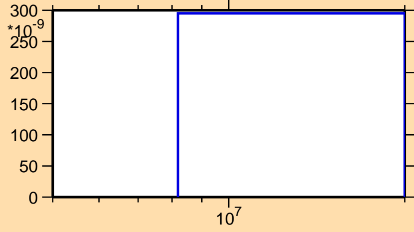
\sigma vs. E for ^{150}\text{Pm}(n,2np)
