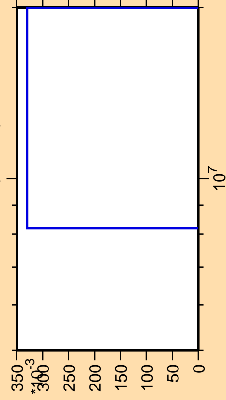
\Delta\sigma/\sigma vs. E for ^{150}\text{Pm}(n,3n\alpha)
