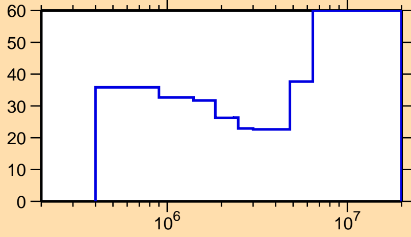
\Delta\sigma/\sigma vs. E for ^{150}\text{Pm}(n,inel.)
