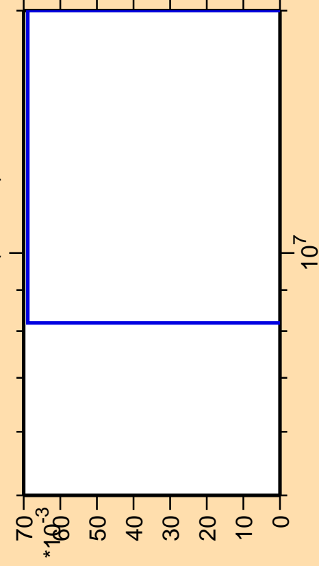
\Delta\sigma/\sigma vs. E for ^{150}\text{Pm} (mt 11)
