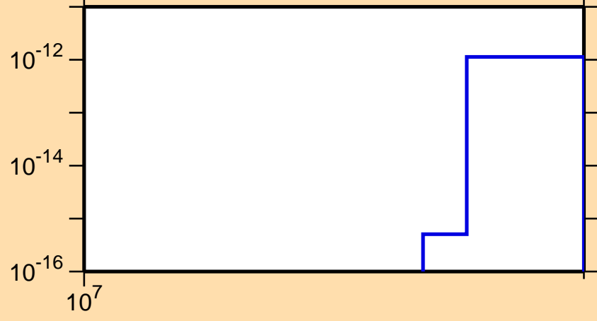
\sigma vs. E for ^{151}\text{Pm}(n,\text{He}3)
