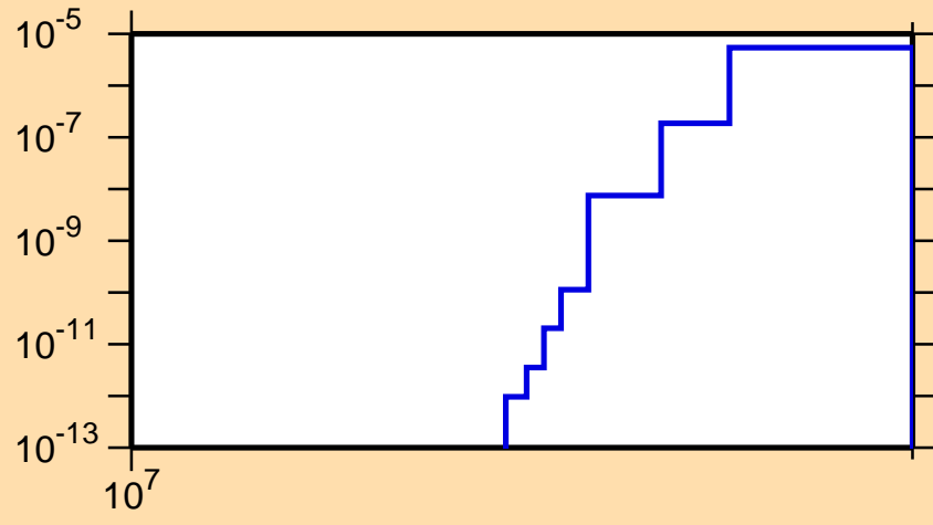
\sigma vs. E for ^{151}\text{Pm}(n,nt)
