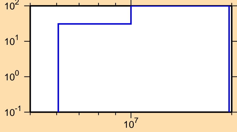
\Delta\sigma/\sigma vs. E for ^{151}\text{Pm}(n,\text{inel.})
