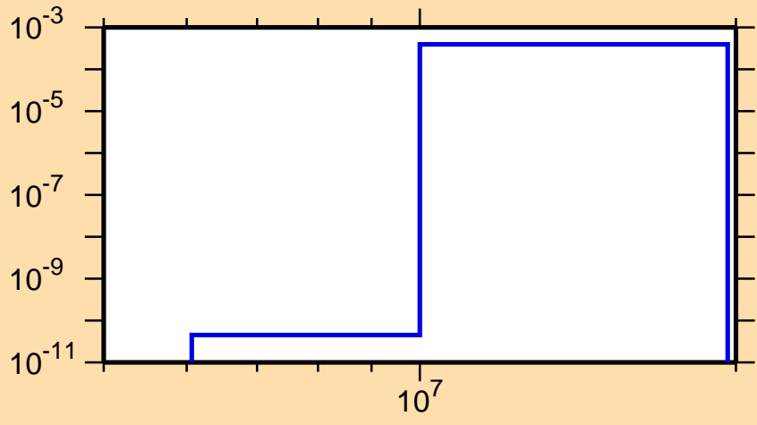
\sigma vs. E for ^{151}\text{Pm}(n,np)
