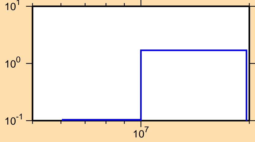
\sigma vs. E for ^{151}\text{Pm}(n,2n)
