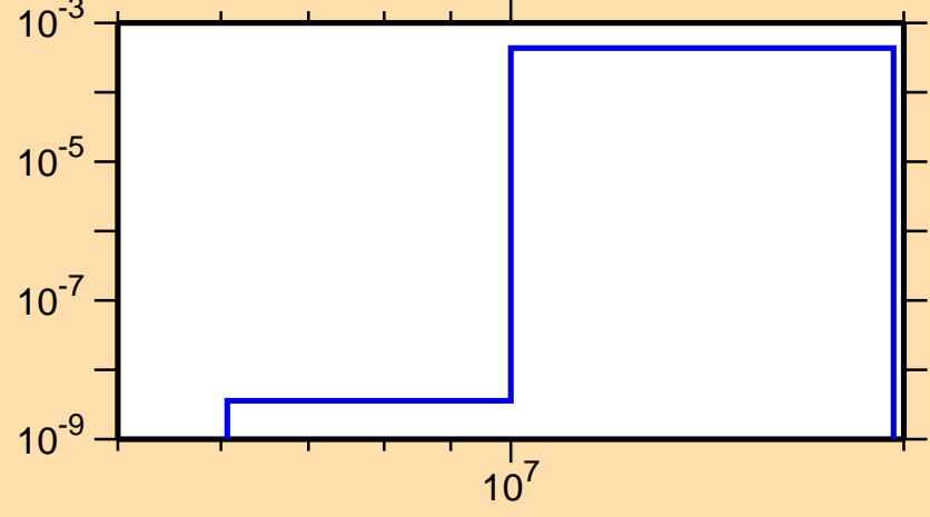
\sigma vs. E for ^{151}\text{Pm}(n,d)
