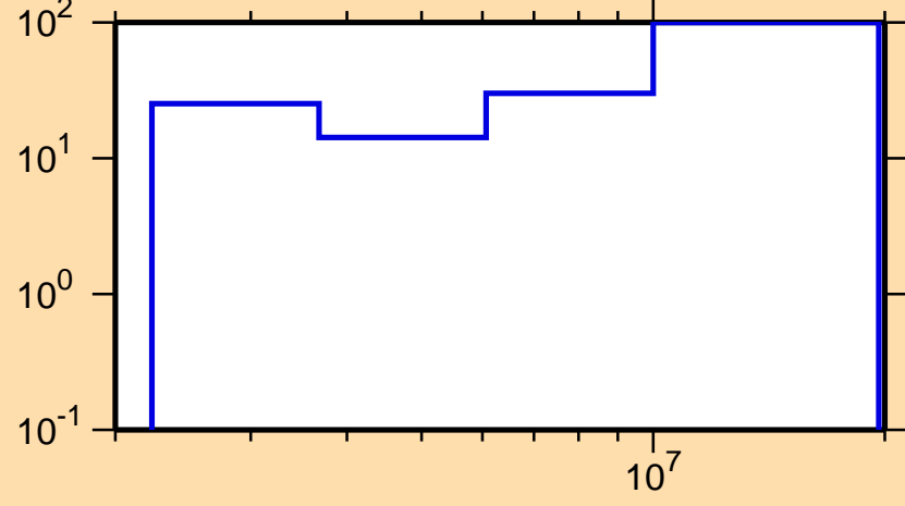
\Delta\sigma/\sigma vs. E for ^{151}\text{Pm}(n,ncont.)
