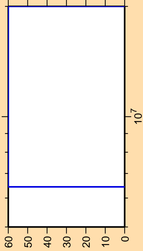
\Delta\sigma/\sigma vs. E for ^{151}\text{Pm}(n,n_1)
