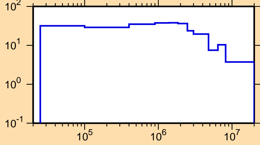
\Delta\sigma/\sigma vs. E for ^{151}\text{Pm}(n,\text{nonel.})
