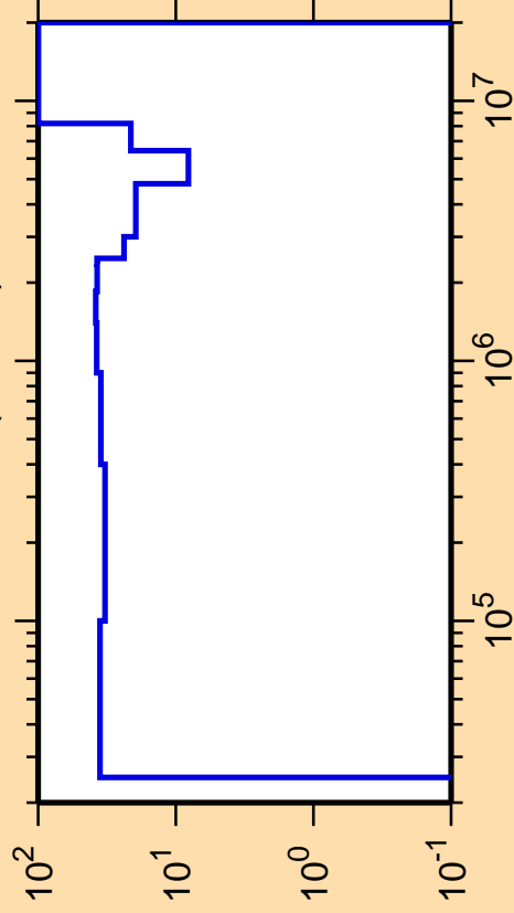
\Delta\sigma/\sigma vs. E for ^{151}\text{Pm}(n,\text{inel.})
