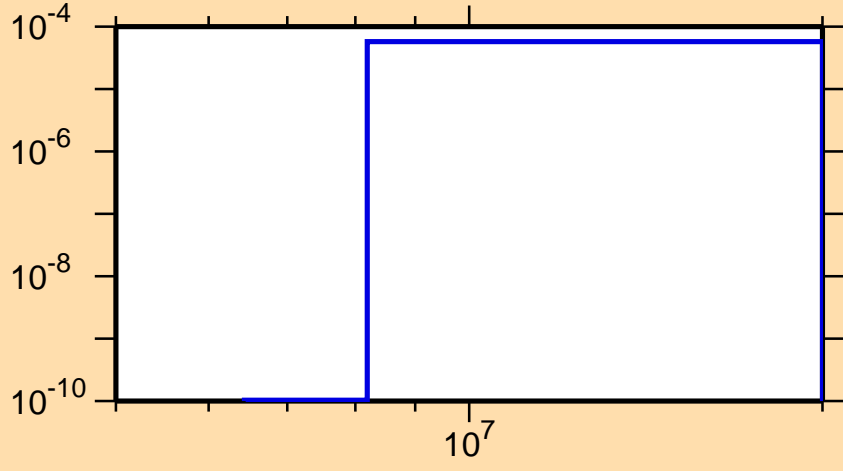
\sigma vs. E for ^{151}\text{Pm}(n,n\alpha)
