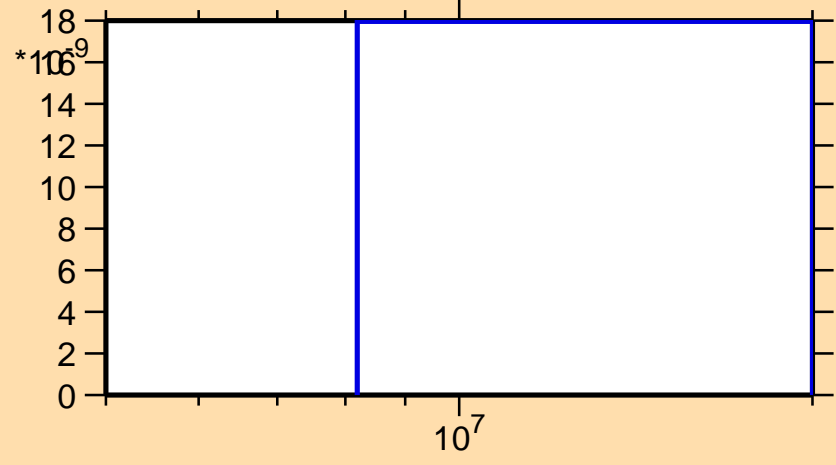
\sigma vs. E for ^{151}\text{Pm}(n,nd)
