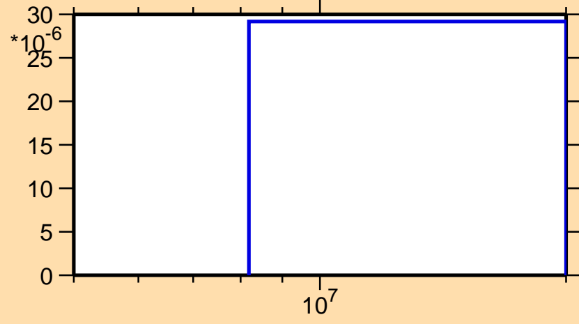
\sigma vs. E for ^{151}\text{Pm}(n,t)
