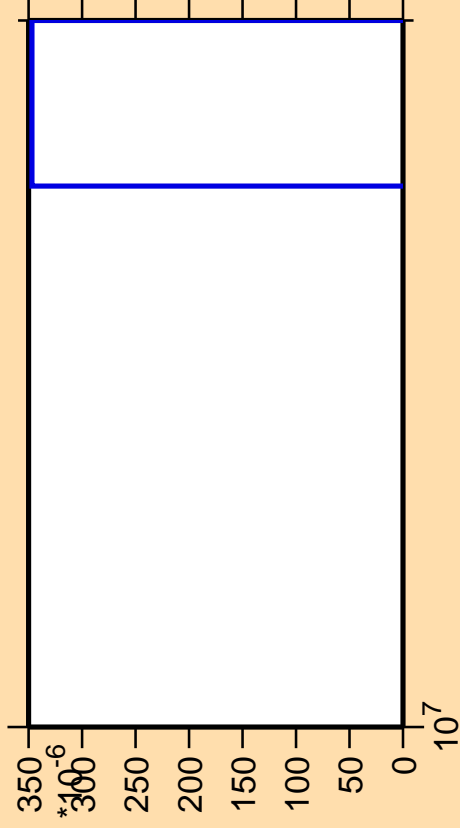
\Delta\sigma/\sigma vs. E for ^{152}\text{Pm} (mt 11)
