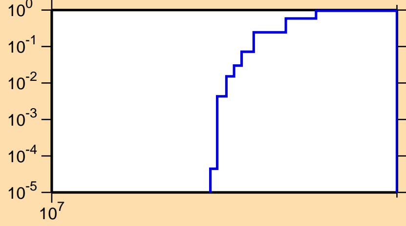
\sigma vs. E for ^{152}\text{Pm}(n,3n)
