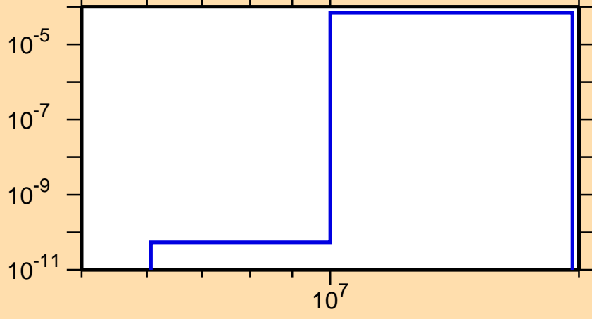
\sigma vs. E for ^{152}\text{Pm}(n,t)
