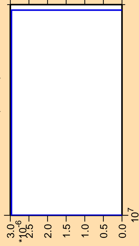
\Delta\sigma/\sigma vs. E for ^{152}\text{Pm} (mt 11)
