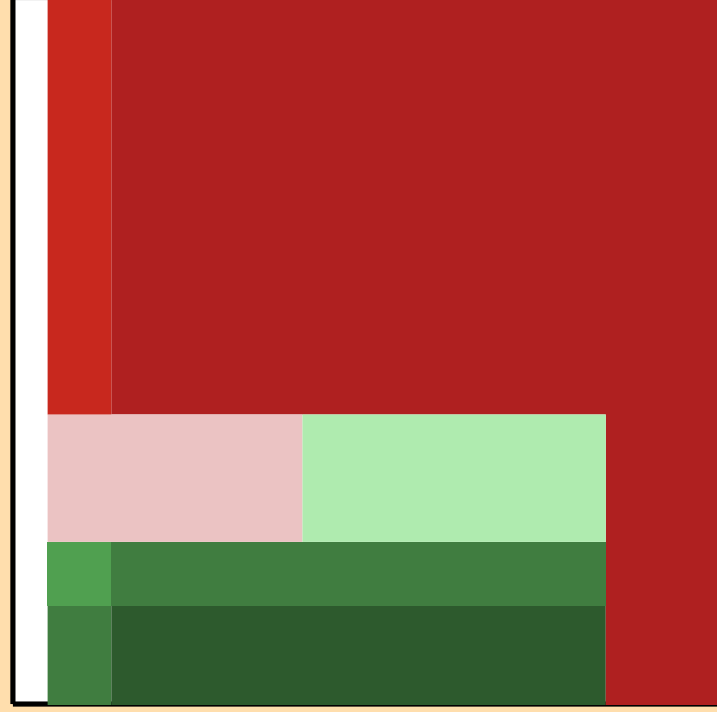
\Delta\sigma/\sigma vs. E for ^{152}\text{Pm}(n,2n)
