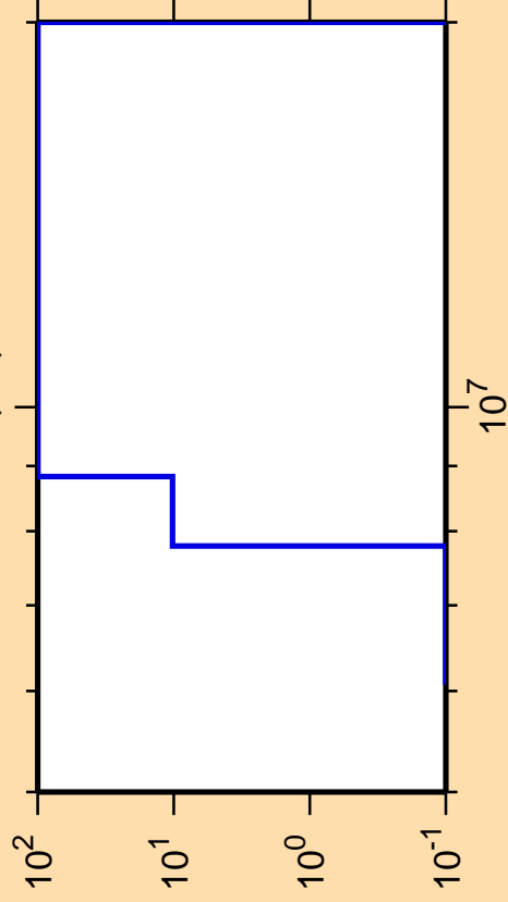
\Delta\sigma/\sigma vs. E for ^{152}\text{Pm}(n,t)
