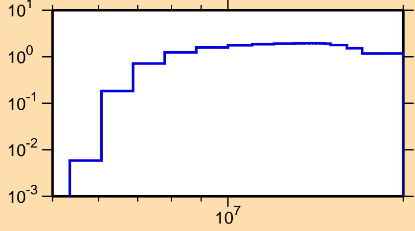
\sigma vs. E for ^{152}\text{Pm}(n,2n)
