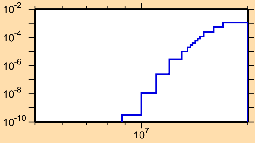
\sigma vs. E for ^{152}\text{Pm}(n,t)
