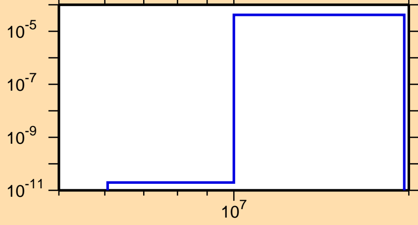
\sigma vs. E for ^{152}\text{Pm}(n,n\alpha)
