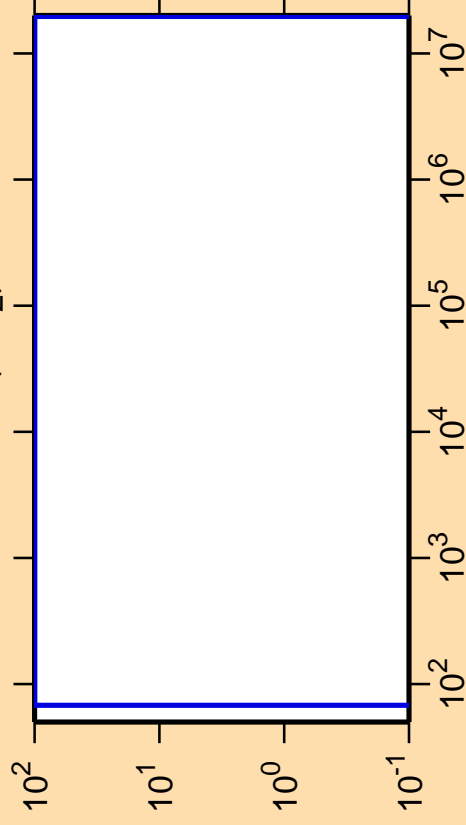
\Delta\sigma/\sigma vs. E for ^{152}\text{Pm}(n,n_2)
