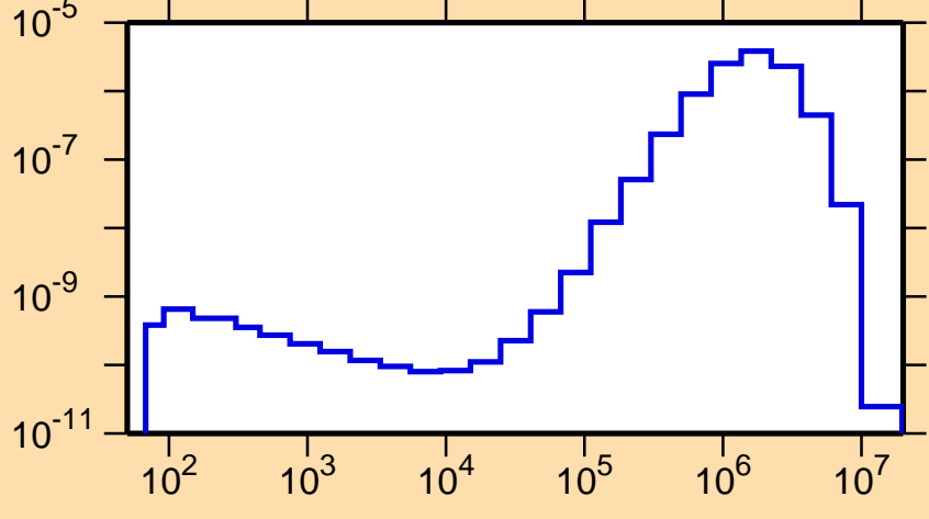
\sigma vs. E for ^{152}\text{Pm}(n,n_2)
