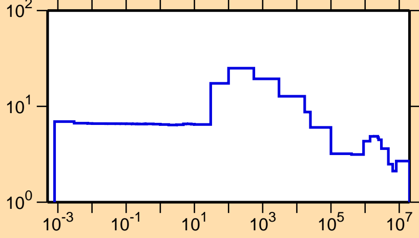
\sigma vs. E for ^{152}\text{Pm}(n,\text{el.})
