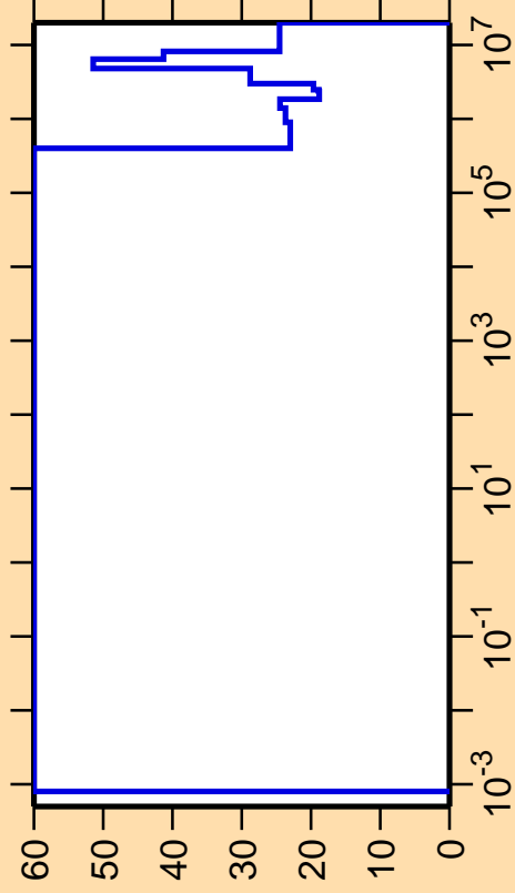
\Delta\sigma/\sigma vs. E for ^{152}\text{Pm}(n,\text{el.})
