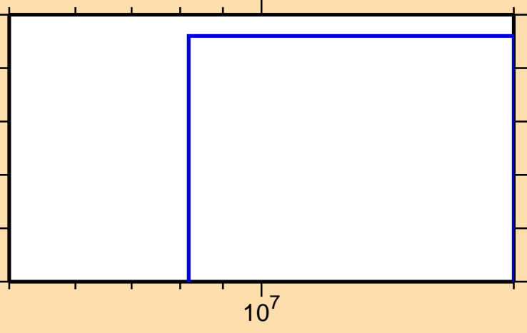
\sigma vs. E for ^{152}\text{Pm}(n,2np)
