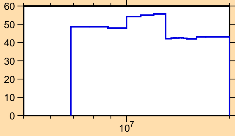
\Delta\sigma/\sigma vs. E for ^{153}\text{Pm}(n,\text{inel.})
