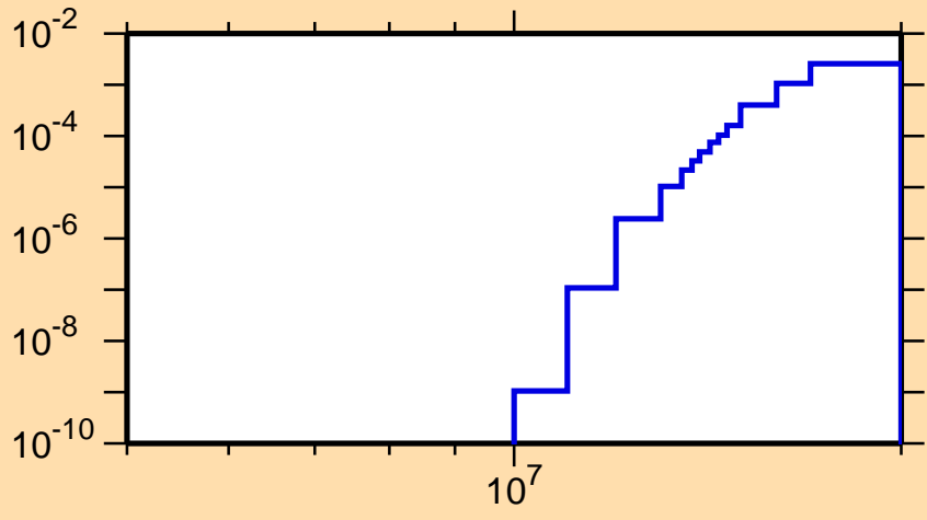
\sigma vs. E for ^{153}\text{Pm}(n,np)
