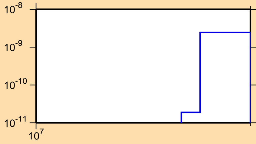
\sigma vs. E for ^{153}\text{Pm}(n,2n\alpha)
