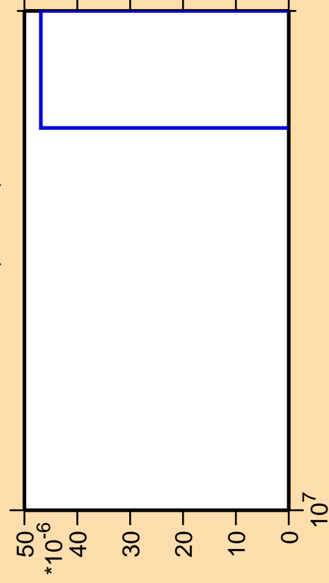
\Delta\sigma/\sigma vs. E for ^{153}\text{Pm} (mt 11)
