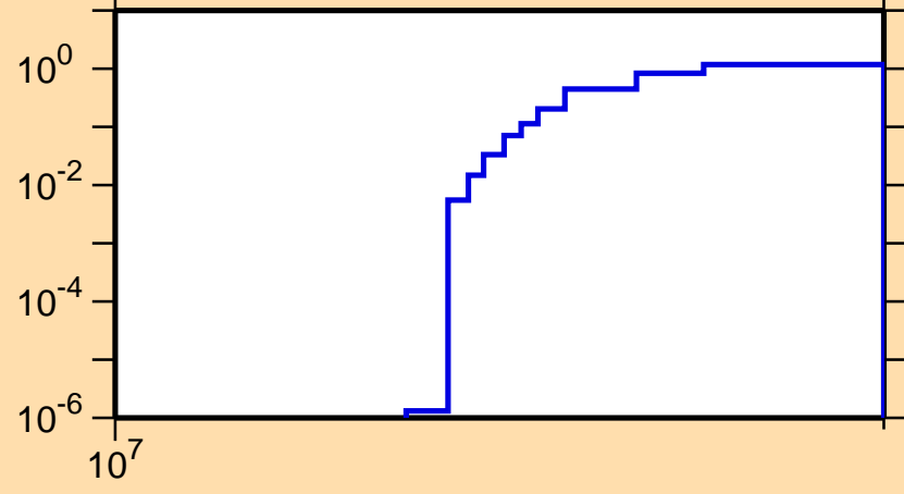
\sigma vs. E for ^{153}\text{Pm}(n,3n)
