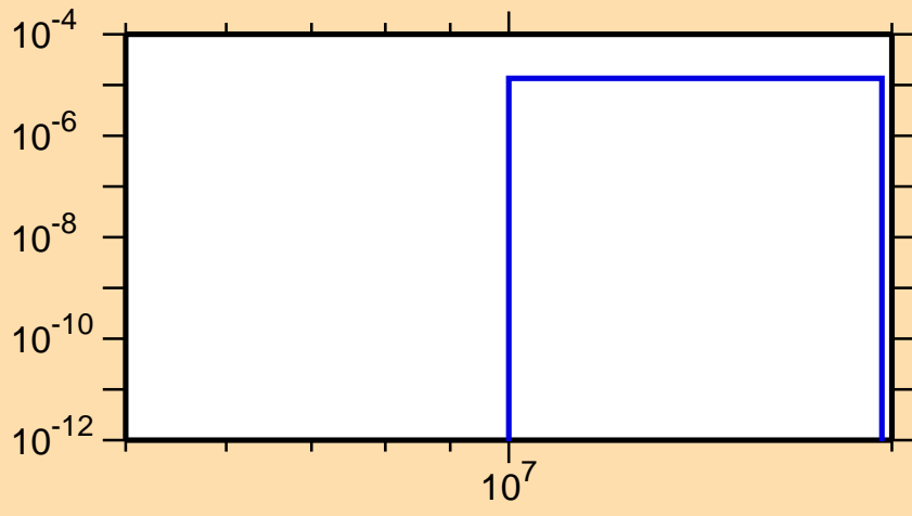
\sigma vs. E for ^{153}\text{Pm}(n,t)
