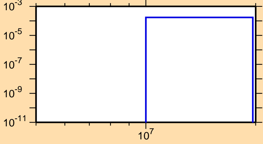
\sigma vs. E for ^{153}\text{Pm}(n,np)
