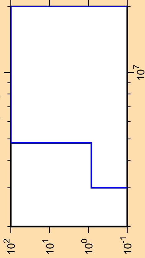
\Delta\sigma/\sigma vs. E for ^{153}\text{Pm}(n,\alpha)
