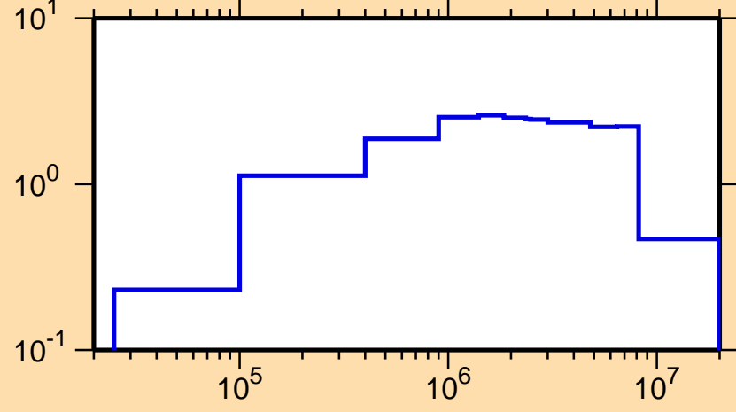
\sigma vs. E for ^{153}\text{Pm}(n,\text{inel.})
