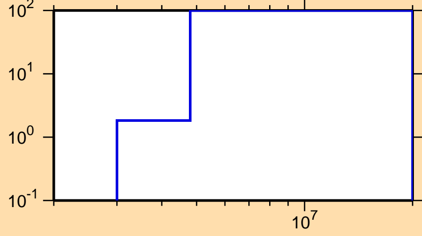
\Delta\sigma/\sigma vs. E for ^{153}\text{Pm}(n,p)
