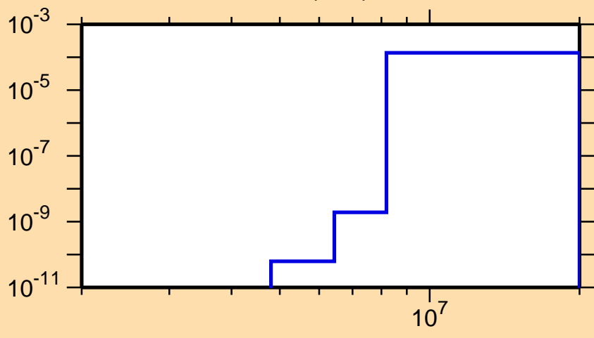
\sigma vs. E for ^{154}\text{Pm}(n,\alpha)
