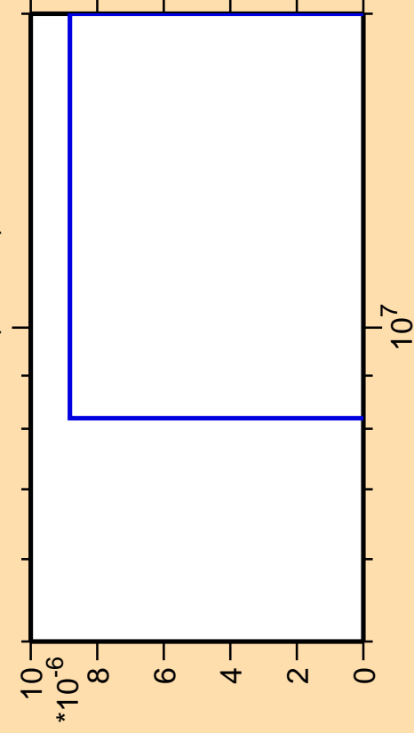
\Delta\sigma/\sigma vs. E for ^{154}\text{Pm} (mt 11)
