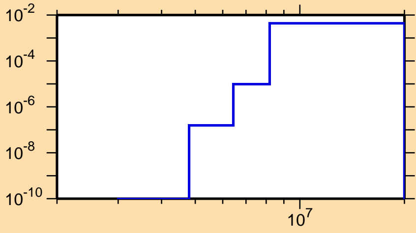
\sigma vs. E for ^{154}\text{Pm}(n,p)
