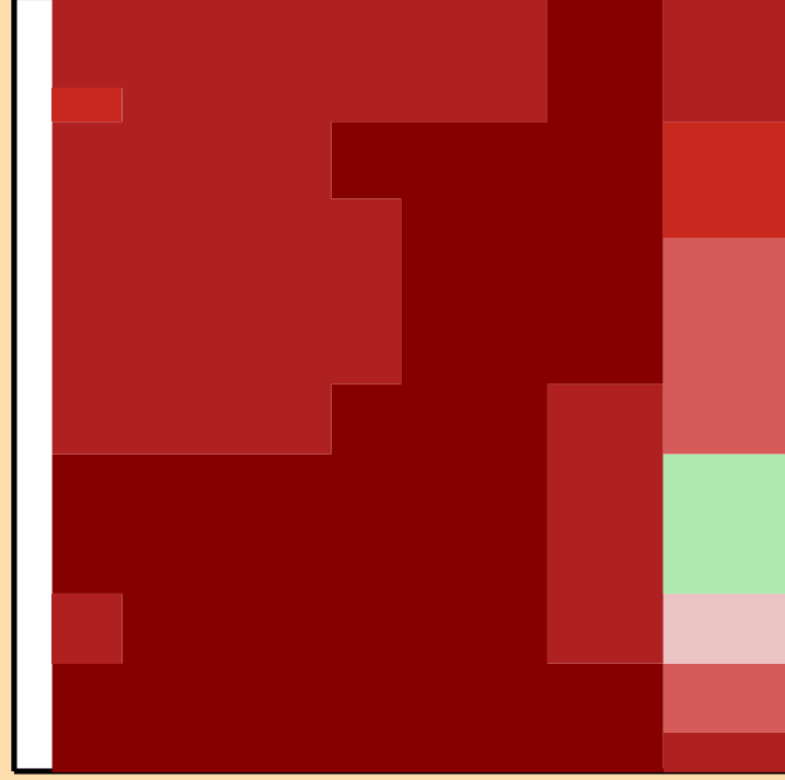
\Delta\sigma/\sigma vs. E for ^{154}\text{Pm}(n,2n)
