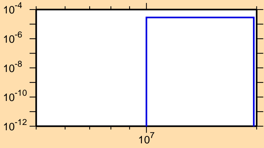
\sigma vs. E for ^{154}\text{Pm}(n,t)
