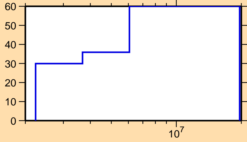
\Delta\sigma/\sigma vs. E for ^{154}\text{Pm}(n,ncont.)
