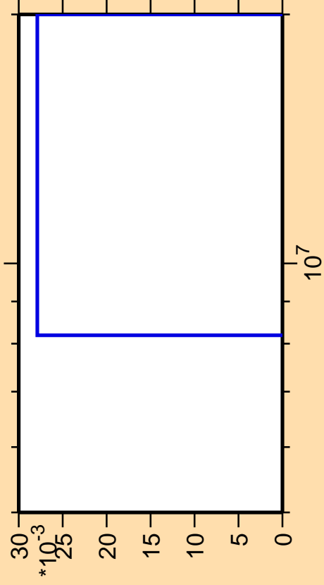
\Delta\sigma/\sigma vs. E for ^{154}\text{Pm}(n,\text{He}3)
