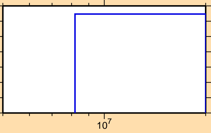
\sigma vs. E for ^{154}\text{Pm}(n,2np)
