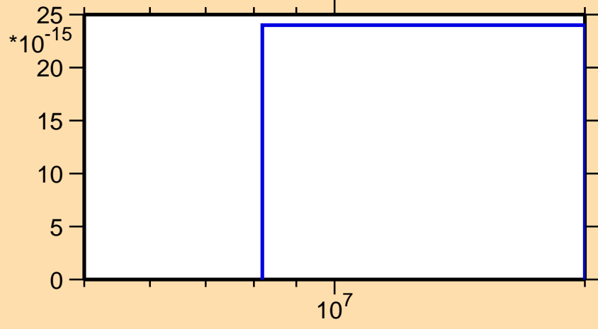
\sigma vs. E for ^{154}\text{Pm}(n,\text{He}3)
