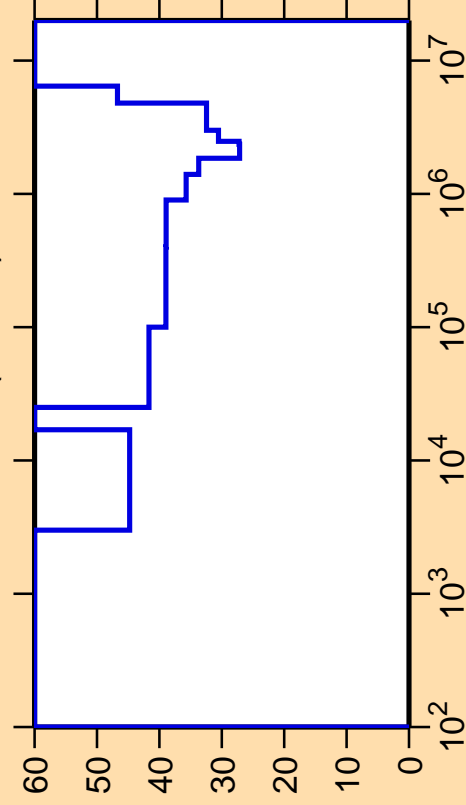
\Delta\sigma/\sigma vs. E for ^{154}\text{Pm}(n,\text{inel.})
