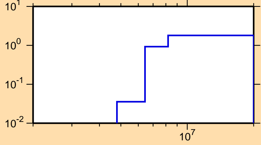
\sigma vs. E for ^{154}\text{Pm}(n,2n)
