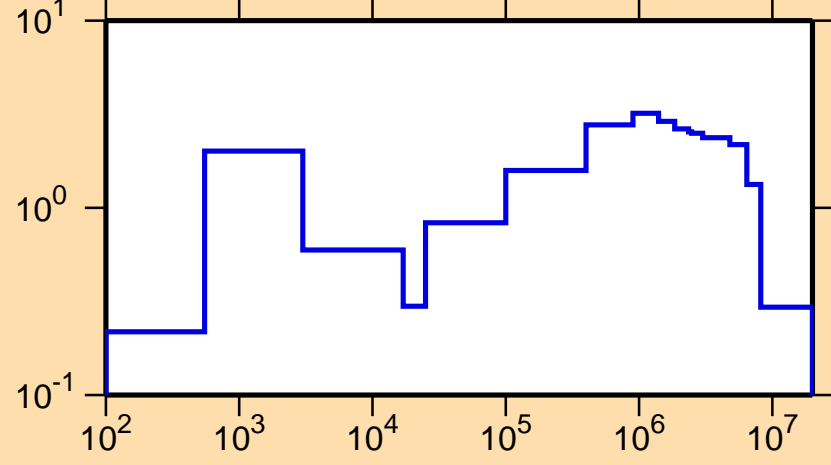
\sigma vs. E for ^{154}\text{Pm}(n,\text{inel.})
