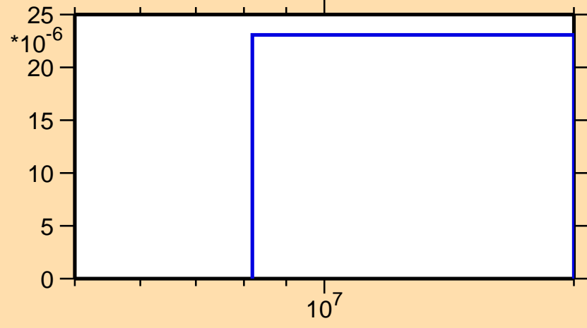
\sigma vs. E for ^{154}\text{Pm}(n,t)
