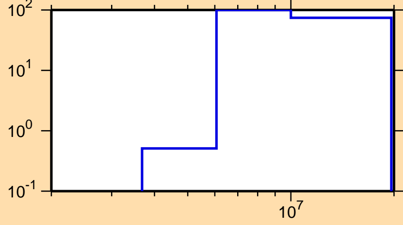
\Delta\sigma/\sigma vs. E for ^{155}\text{Pm}(n,p)
