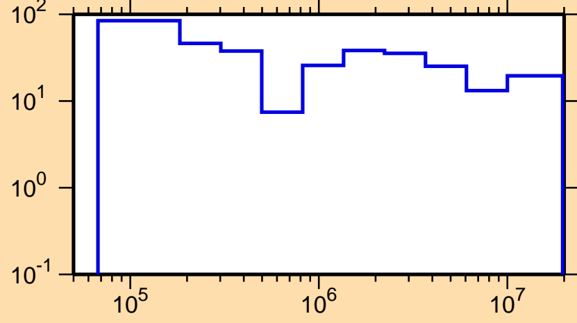
\Delta\sigma/\sigma vs. E for ^{155}\text{Pm}(n,\text{tot.})
