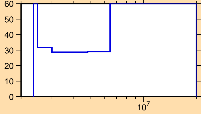
\Delta\sigma/\sigma vs. E for ^{155}\text{Pm}(n,n\text{cont.})
