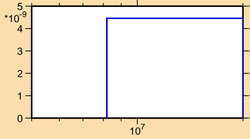
\sigma vs. E for ^{155}\text{Pm}(n,\text{nd})
