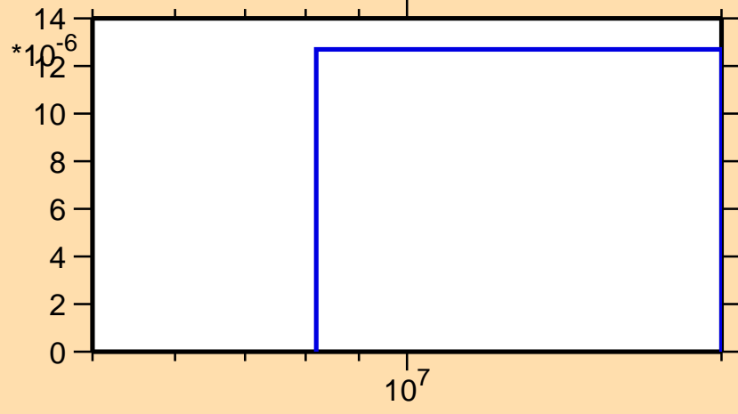
\sigma vs. E for ^{155}\text{Pm}(n,t)
