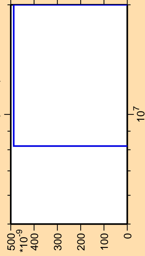
\Delta\sigma/\sigma vs. E for ^{155}\text{Pm}(\text{mt } 11)
