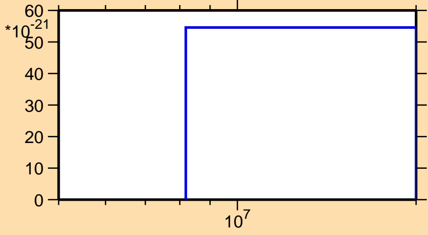
\sigma vs. E for ^{155}\text{Pm}(\text{mt } 11)
