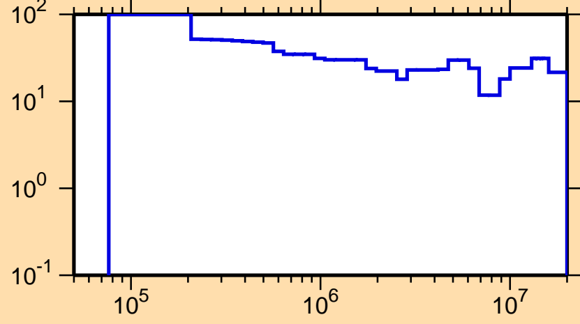
\Delta\sigma/\sigma vs. E for ^{156}\text{Pm}(n,\text{el.})
