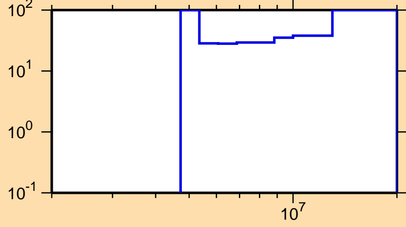
\Delta\sigma/\sigma vs. E for ^{156}\text{Pm}(n,2n)
