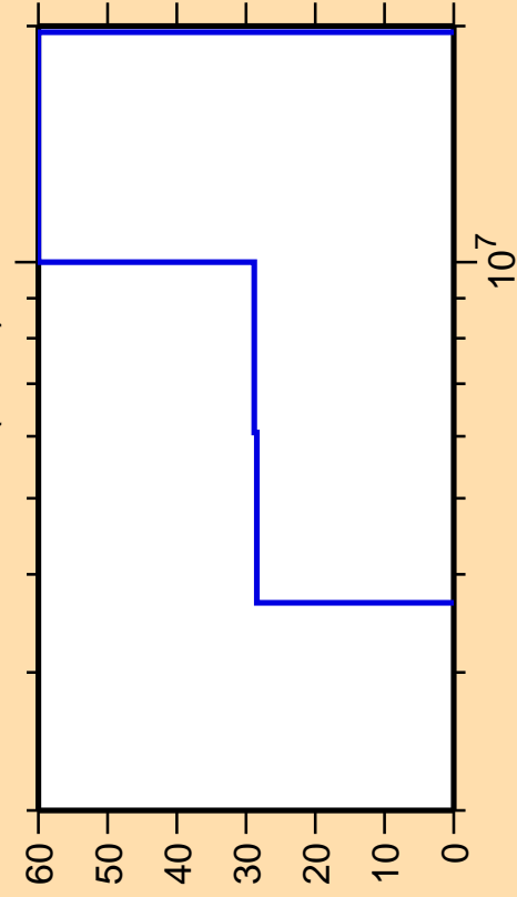
\Delta\sigma/\sigma vs. E for ^{156}\text{Pm}(n,2n)
