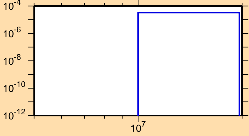
\sigma vs. E for ^{156}\text{Pm}(n,np)
