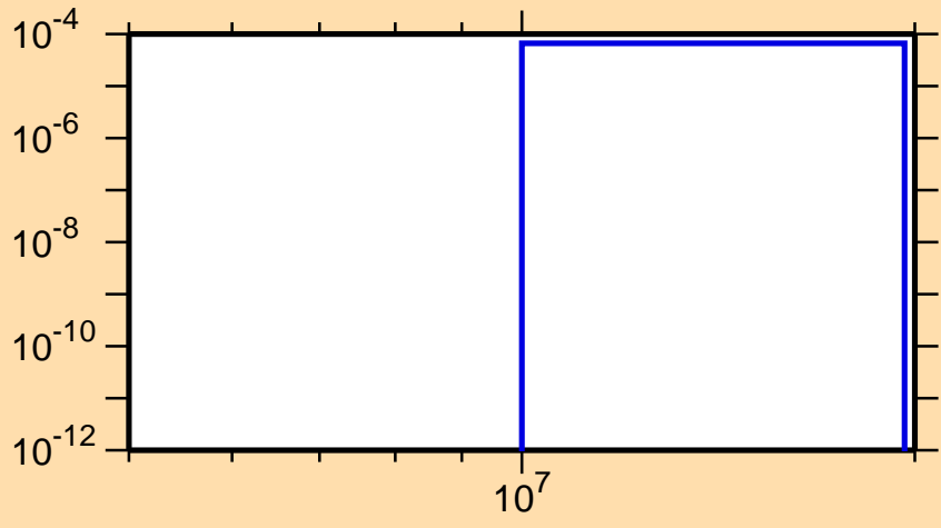
\sigma vs. E for ^{156}\text{Pm}(n,d)
