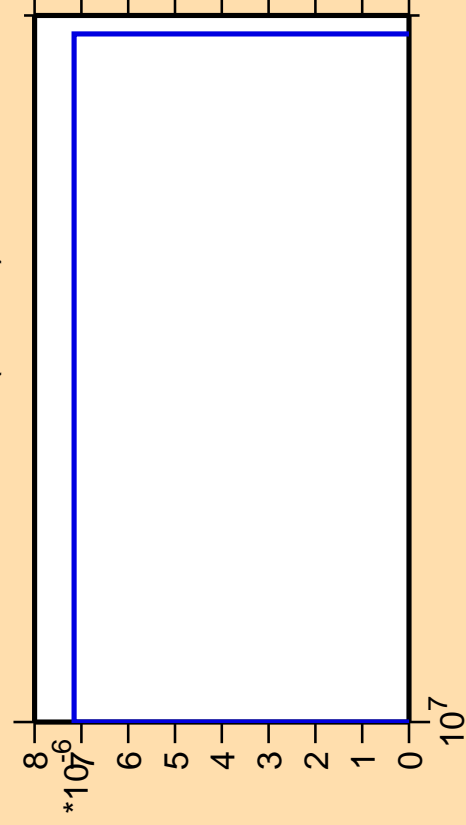
\Delta\sigma/\sigma vs. E for ^{156}\text{Pm} (mt 11)
