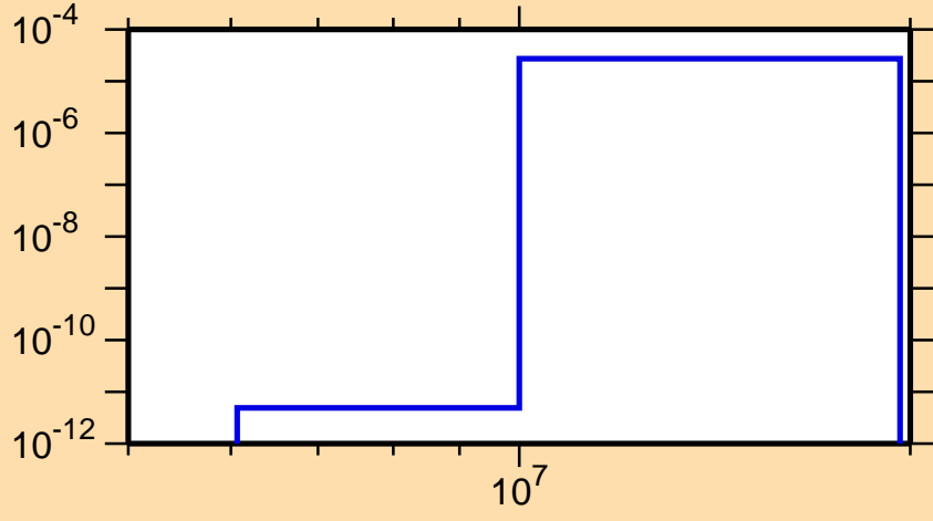
\sigma vs. E for ^{156}\text{Pm}(n,t)
