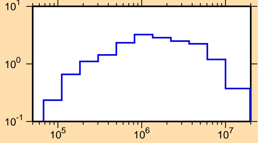
\sigma vs. E for ^{156}\text{Pm}(n,\text{inel.})
