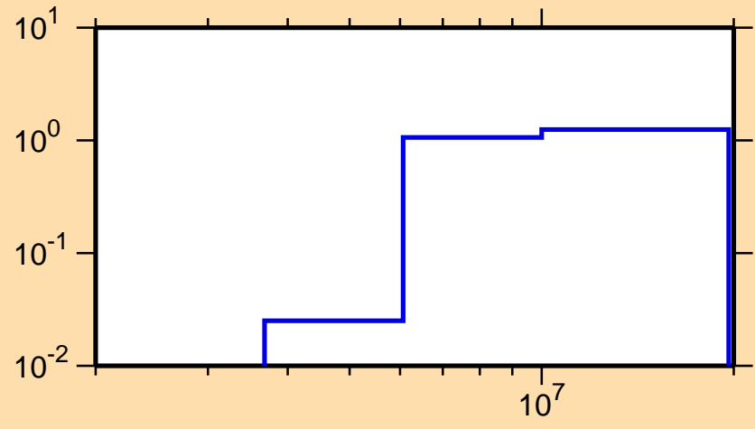
\sigma vs. E for ^{156}\text{Pm}(n,2n)
