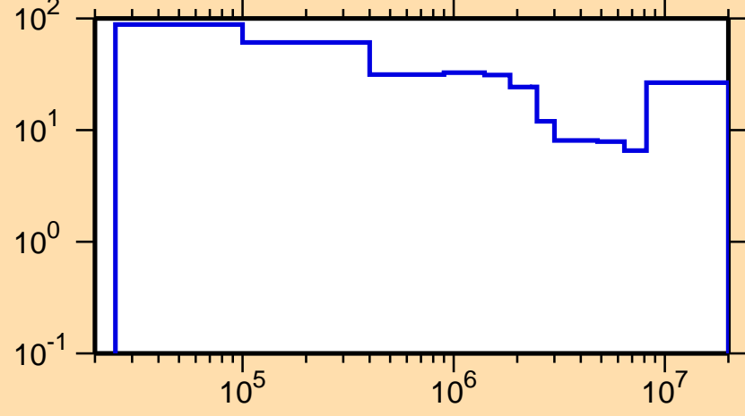
\Delta\sigma/\sigma vs. E for ^{156}\text{Pm}(n,\text{tot.})
