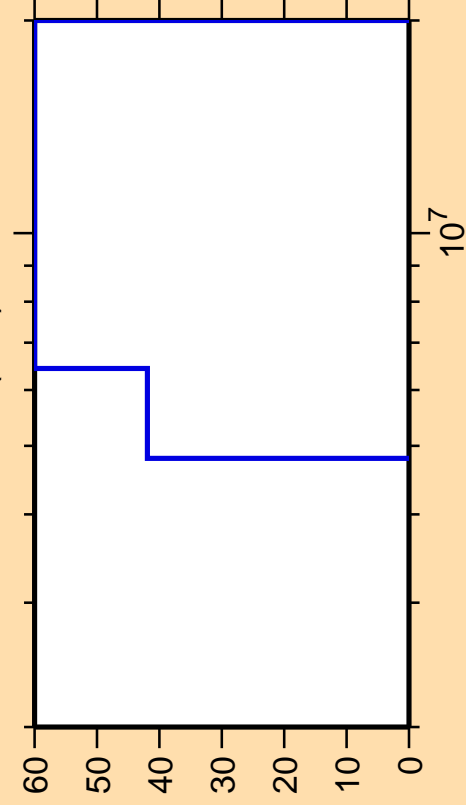
\Delta\sigma/\sigma vs. E for ^{156}\text{Pm}(n,\alpha)
