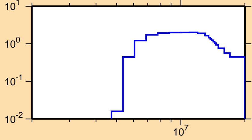
\sigma vs. E for ^{156}\text{Pm}(n,2n)
