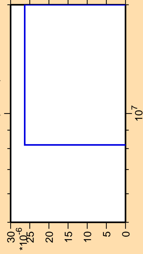
\Delta\sigma/\sigma vs. E for ^{156}\text{Pm}(\text{mt } 11)
