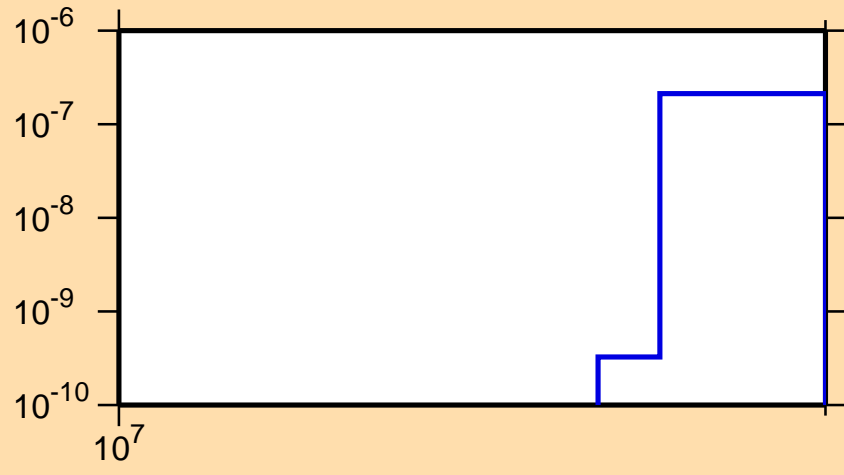
\sigma vs. E for ^{157}\text{Pm}(n,\text{nd})
