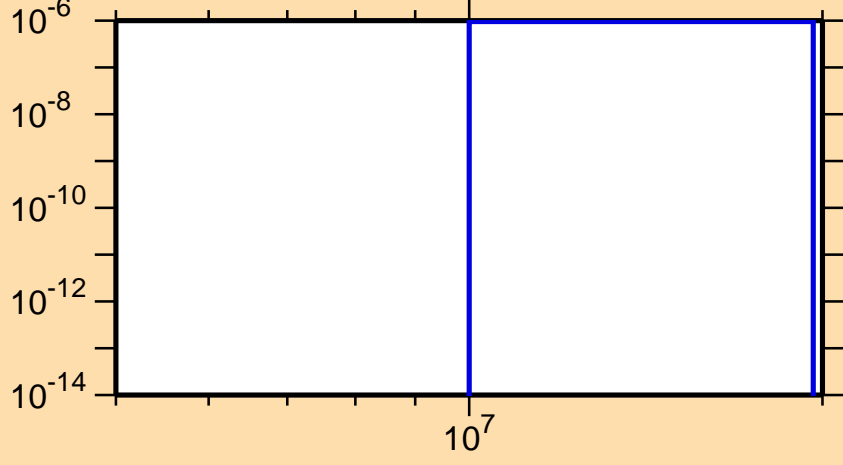
\sigma vs. E for ^{157}\text{Pm}(n,n\alpha)
